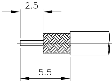
RECOMMENDED CABLE STRIPPING DIM'S
