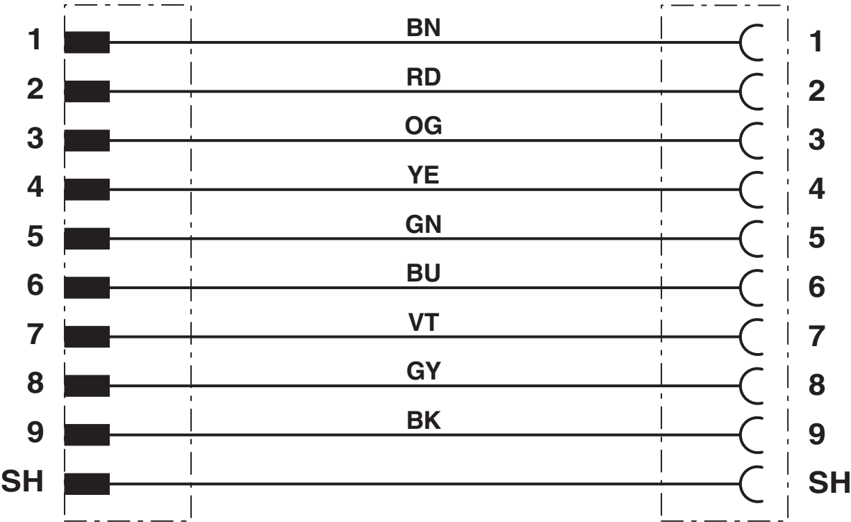
Circuit diagram
