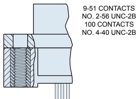
NU Style Threaded Insert
