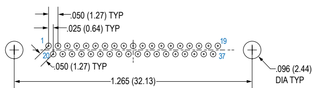
37 Contacts
