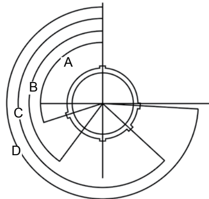
FACE VIEW RECEPTACLE POSITION N, 6 THRU 10
