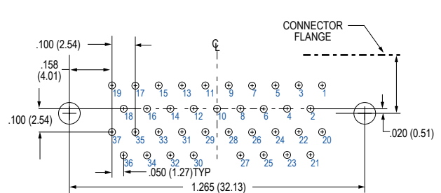
37 Contacts
