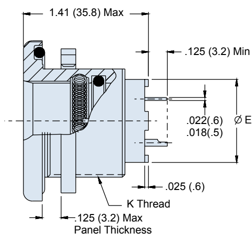
08 - Jam Nut Receptacle, Front Mount, with PCB Stand-Off
