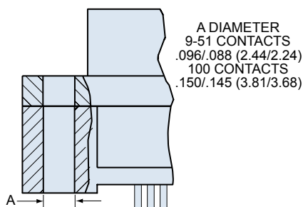
NN Style Thru-Hole, No Hardware
