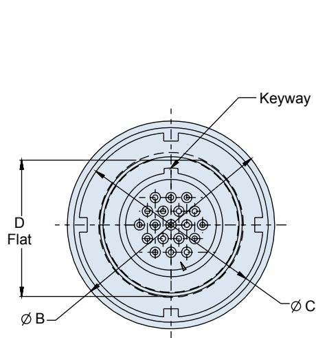
07 - Jam Nut Receptacle, Rear Mount, with PCB Stand-Off
