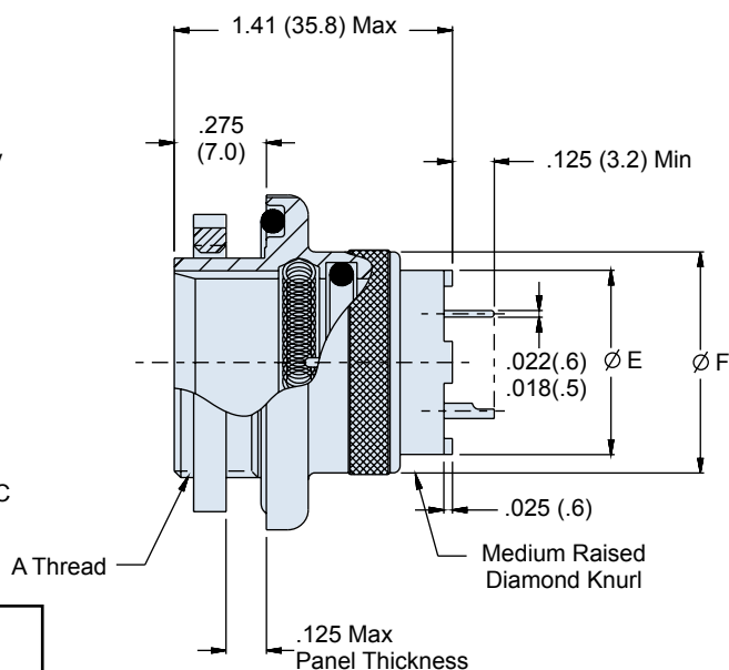
07 - Jam Nut Receptacle, Rear Mount, with PCB Stand-Off
