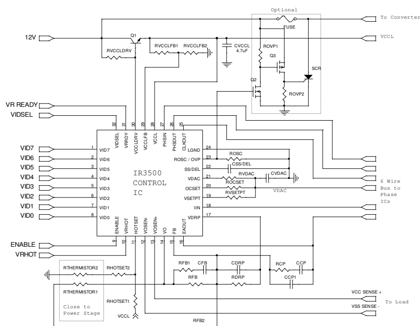
Figure 1 – Application Circuit
