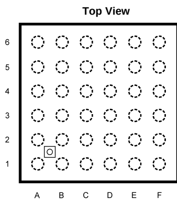
Connection Diagrams
