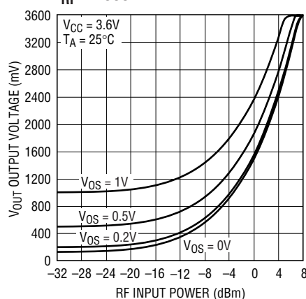
V_{OUT} vs RF Input Power and V_{OS} , f_{RF} = 1000MHz
