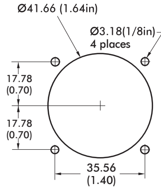
DROP-IN, RAISED, SNAP-ON REAR MOUNT OPTION B
