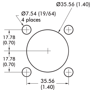
REAR MOUNT OPTION A **
