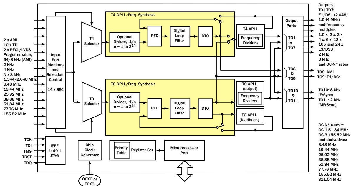
Figure 1 Block Diagram of the ACS8520A SETS
