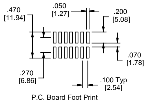
P.C. Board Foot Print
