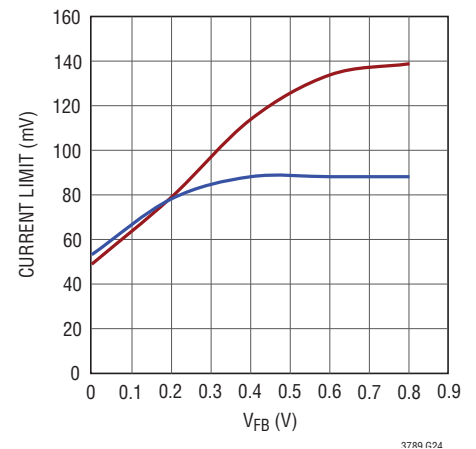
Current Foldback Limit
