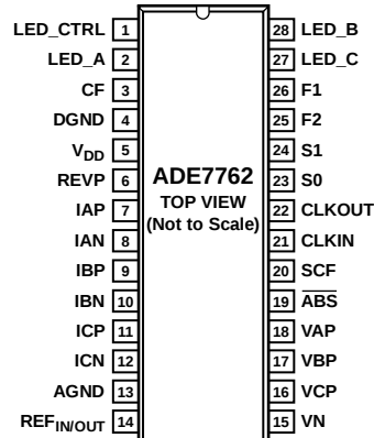
Figure 4. Pin Configuration
