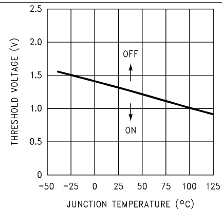
Figure 12. \overline{\text{ON}} /OFF Threshold Voltage
