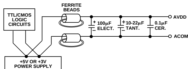
Figure 36. Differential LC Filter for Single +5 V or +3 V Applications
