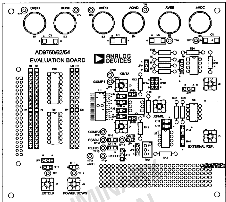
Figure 40. Silkscreen Layer—Top
