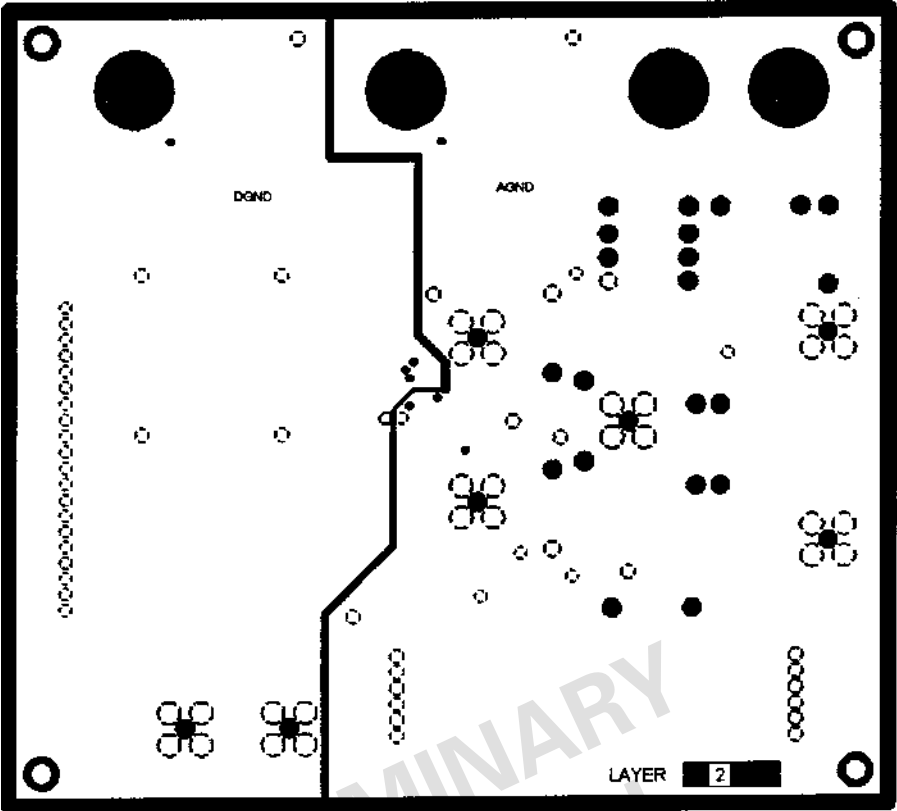
Figure 42. Ground Plane PCB Layout (Layer 2)
