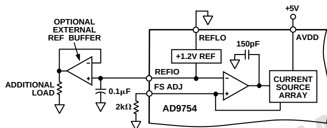
Figure 22. Internal Reference Configuration
