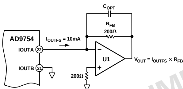
Figure 35. Unipolar Buffered Voltage Output
