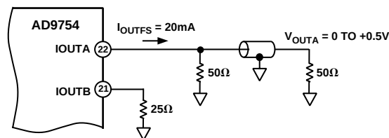
Figure 34. 0 V to +0.5 V Unbuffered Voltage Output
