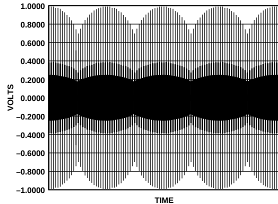
Figure 37b. Time Domain "Snapshot" of the Multitone Waveform
