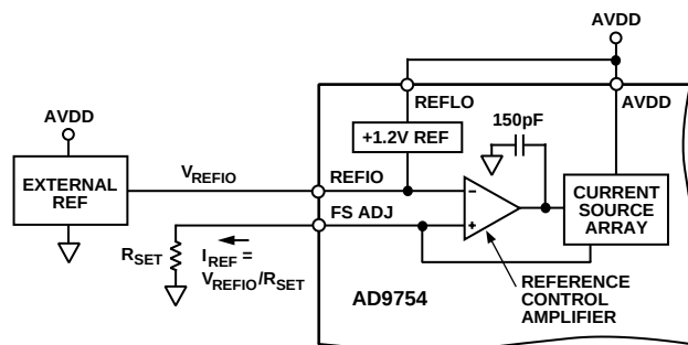
Figure 23. External Reference Configuration
