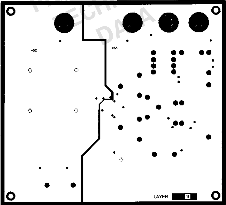
Figure 43. Power Plane PCB Layout (Layer 3)
