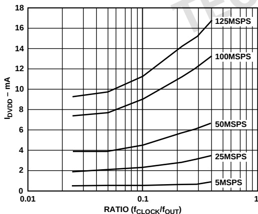
Figure 29. I_{DVDD} vs. Ratio @ DVDD = 5 V
