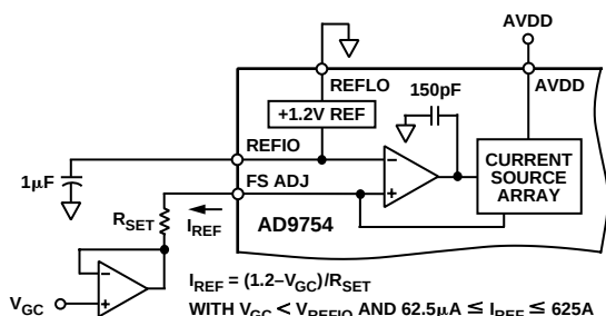
Figure 25. Dual-Supply Gain Control Circuit
