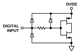
Figure 27. Equivalent Digital Input
