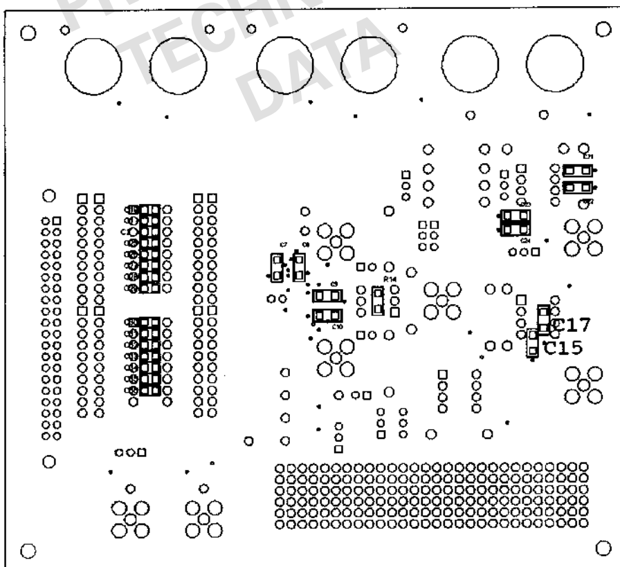
Figure 45. Silkscreen Layer—Bottom
