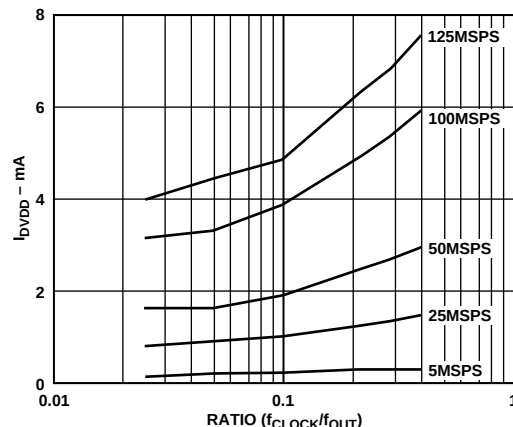
Figure 30. I_{DVDD} vs. Ratio @ DVDD = 3 V
