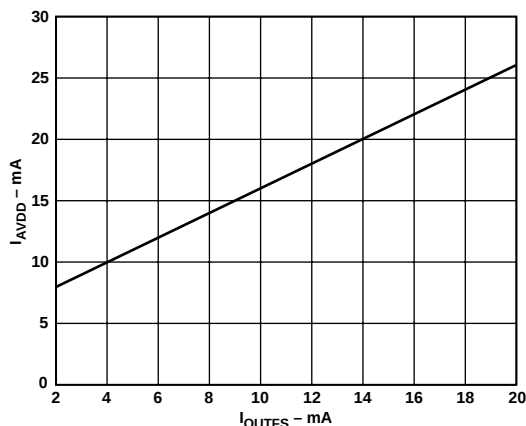
Figure 28. I_{AVDD} vs. I_{OUTFS}
