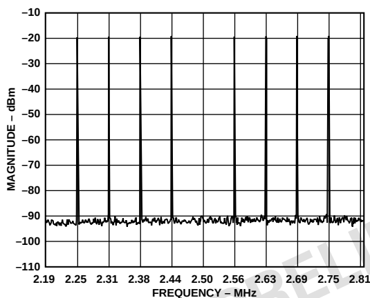
Figure 37a. Multitone Spectral Plot
