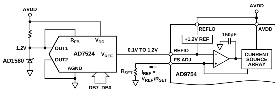
Figure 24. Single-Supply Gain Control Circuit
