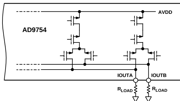
Figure 26. Equivalent Analog Output Circuit
