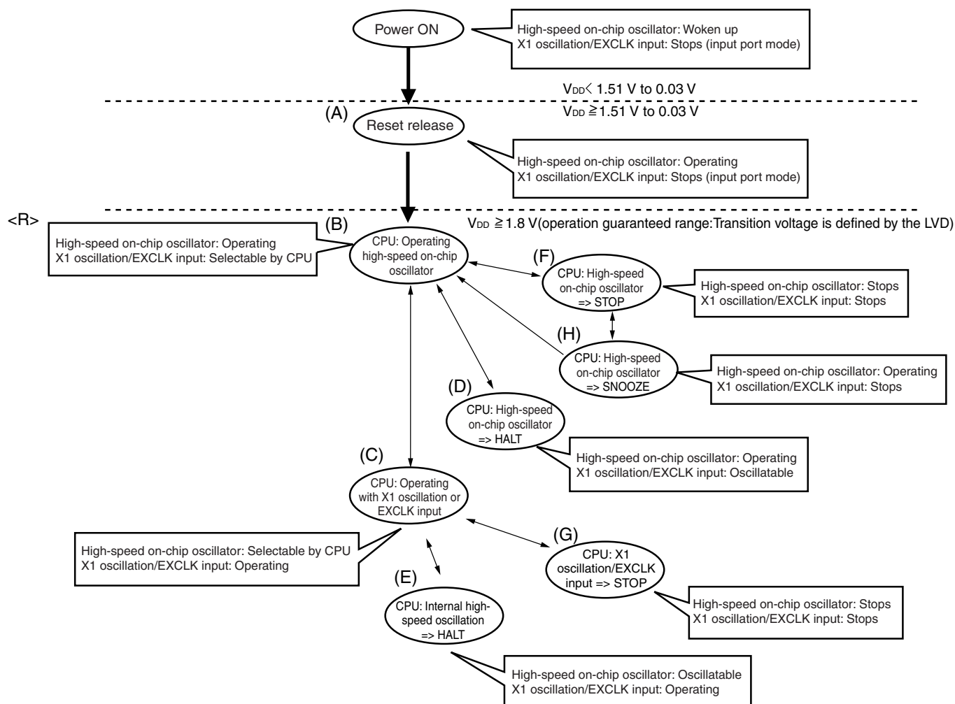
Figure 5-14. CPU Clock Status Transition Diagram
