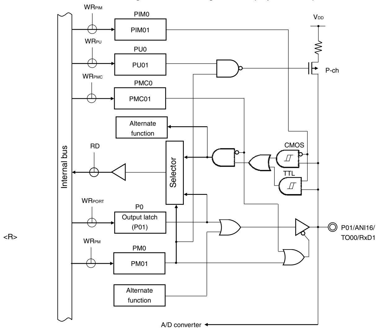
Figure 4-18. Block Diagram of P01 (30-pin Products)
