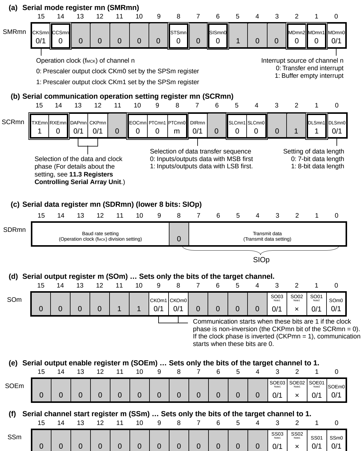
&lt;R&gt; Figure 11-26. Example of Contents of Registers for Master Transmission of 3-Wire Serial I/O (CSI00, CSI01, CSI11, CSI20)
