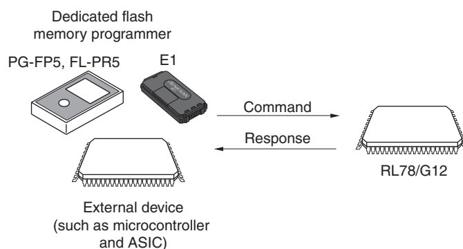
Figure 24-9. Communication Commands
