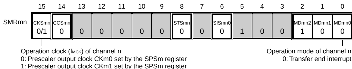
<R> Figure 11-99. Example of Contents of Registers for Address Field Transmission of Simplified I 2 C (IIC00, IIC01, IIC11, IIC20)
