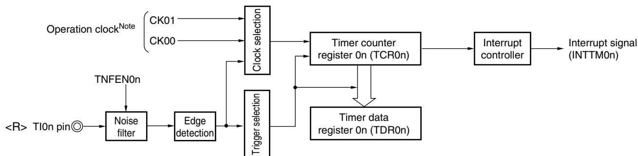
Figure 6-53. Block Diagram of Operation as Input Signal High-/Low-Level Width Measurement
