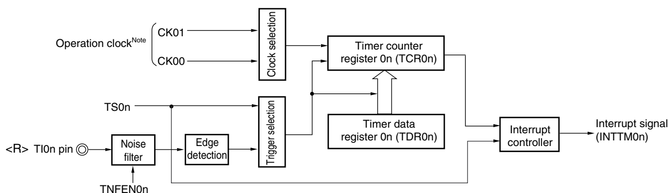
Figure 6-57. Block Diagram of Operation as Delay Counter
