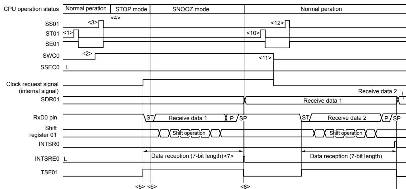
Figure 11-92. Timing Chart of SNOOZE Mode Operation (Abnormal Operation <1>)
