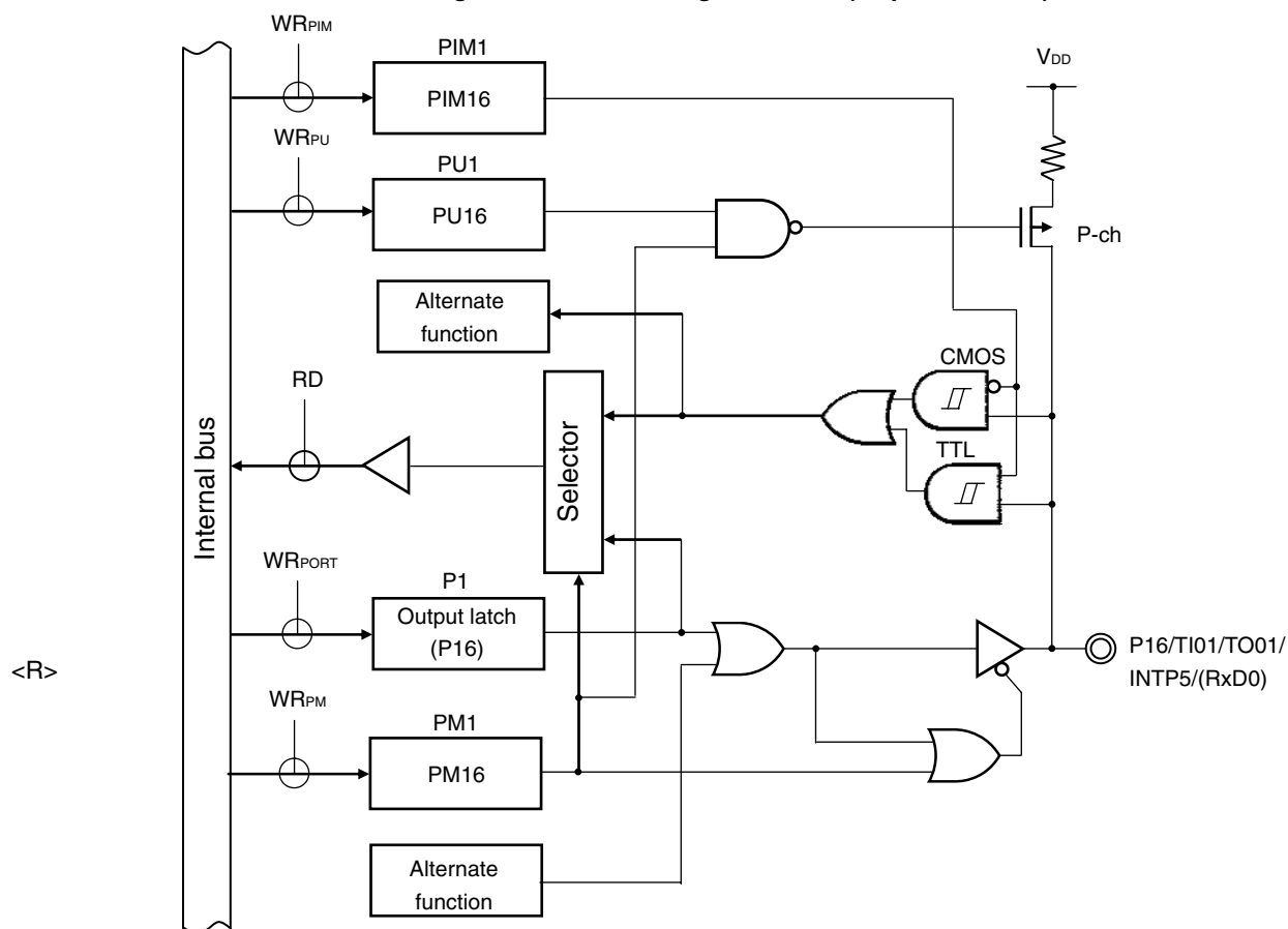
Figure 4-21. Block Diagram of P16 (30-pin Products)
