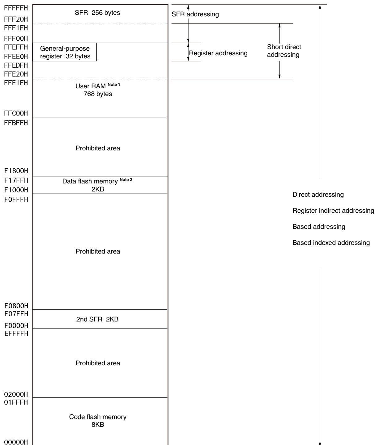
Figure 3-10. Correspondence Between Data Memory and Addressing for the R5F10x68, R5F10x78, and R5F10xA8 (x = 2 or 3)
