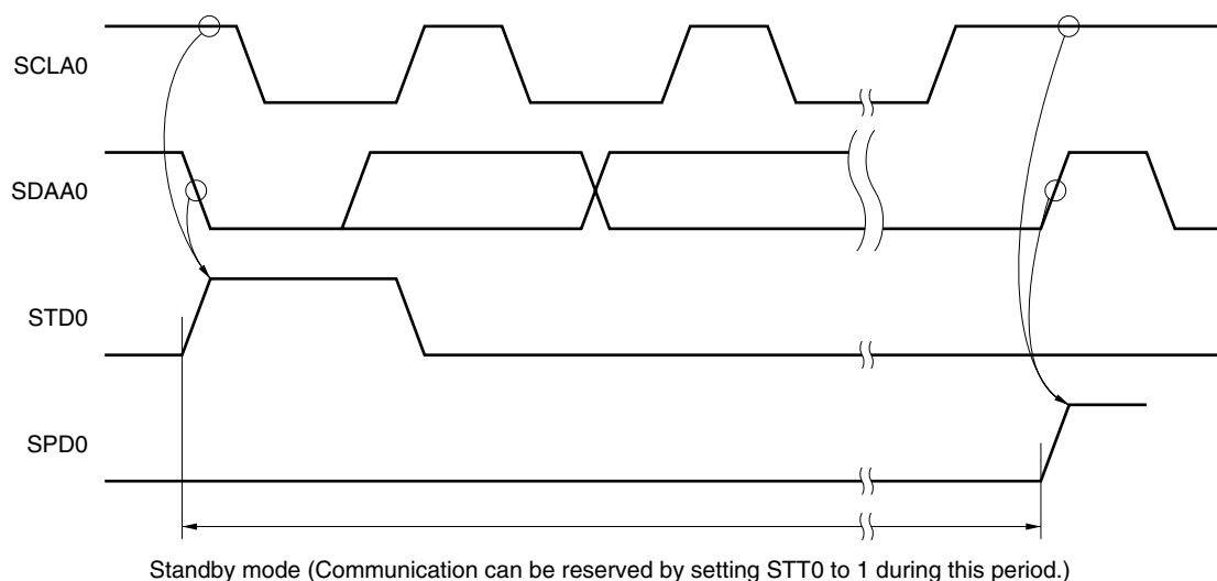
Figure 12-26. Timing for Accepting Communication Reservations
