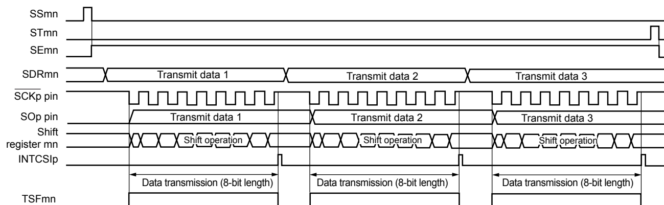
Figure 11-54. Timing Chart of Slave Transmission (in Single-Transmission Mode)
