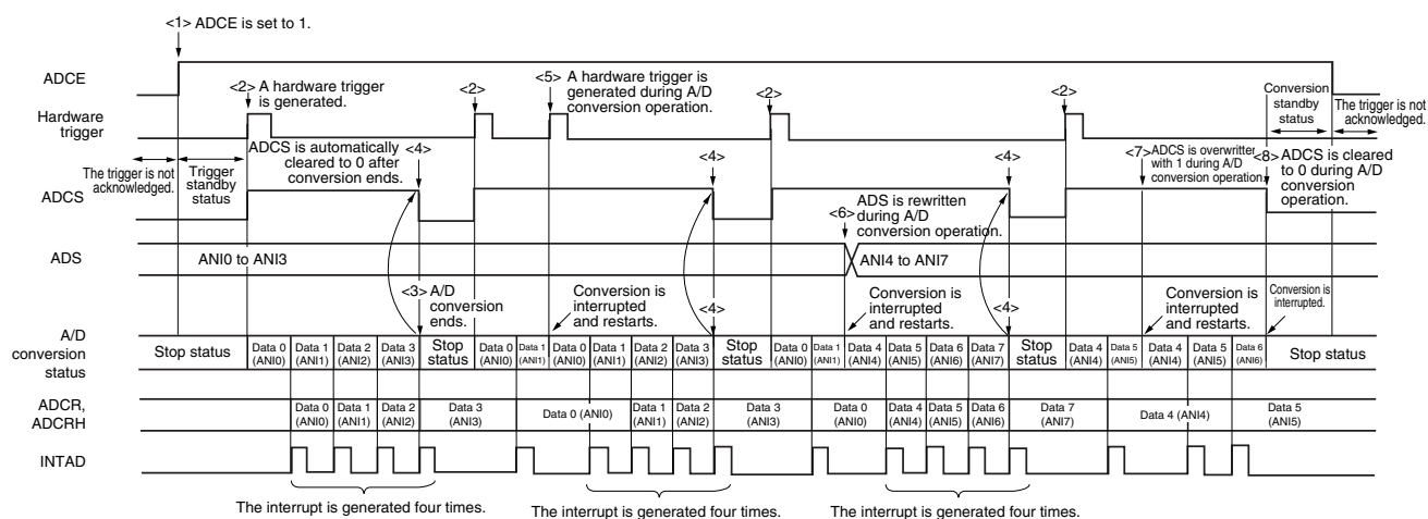
Figure 10-31. Example of Hardware Trigger Wait Mode (Scan Mode, One-Shot Conversion Mode) Operation Timing
