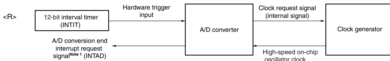
Figure 10-37. Block Diagram When Using SNOOZE Mode Function
