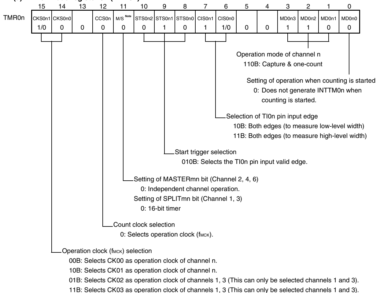
Figure 6-55. Example of Set Contents of Registers to Measure Input Signal High-/Low-Level Width
