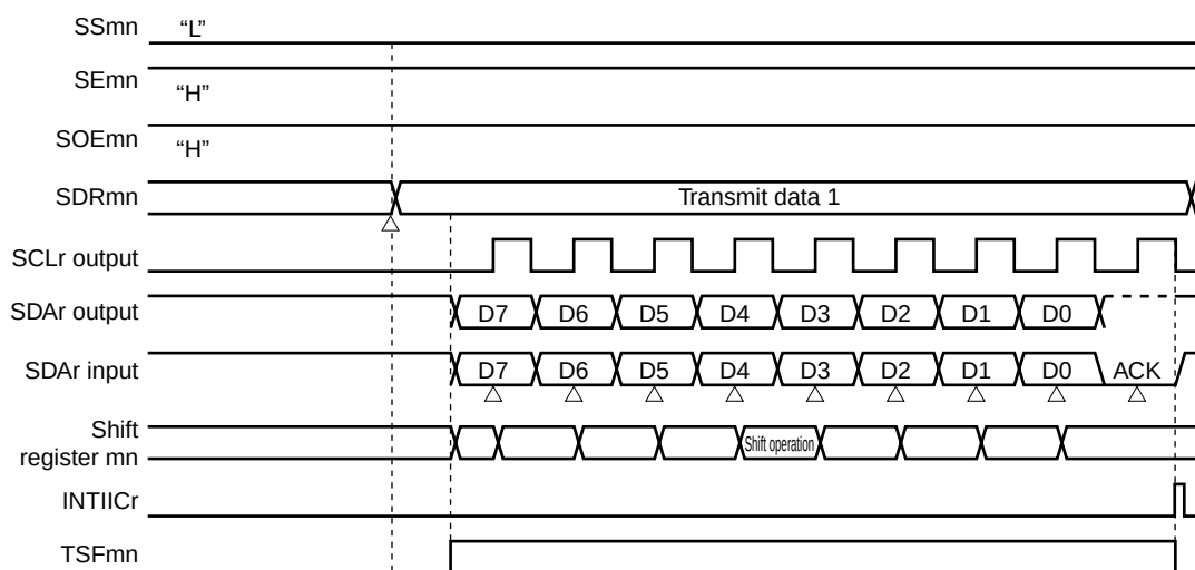
Figure 11-104. Timing Chart of Data Transmission
