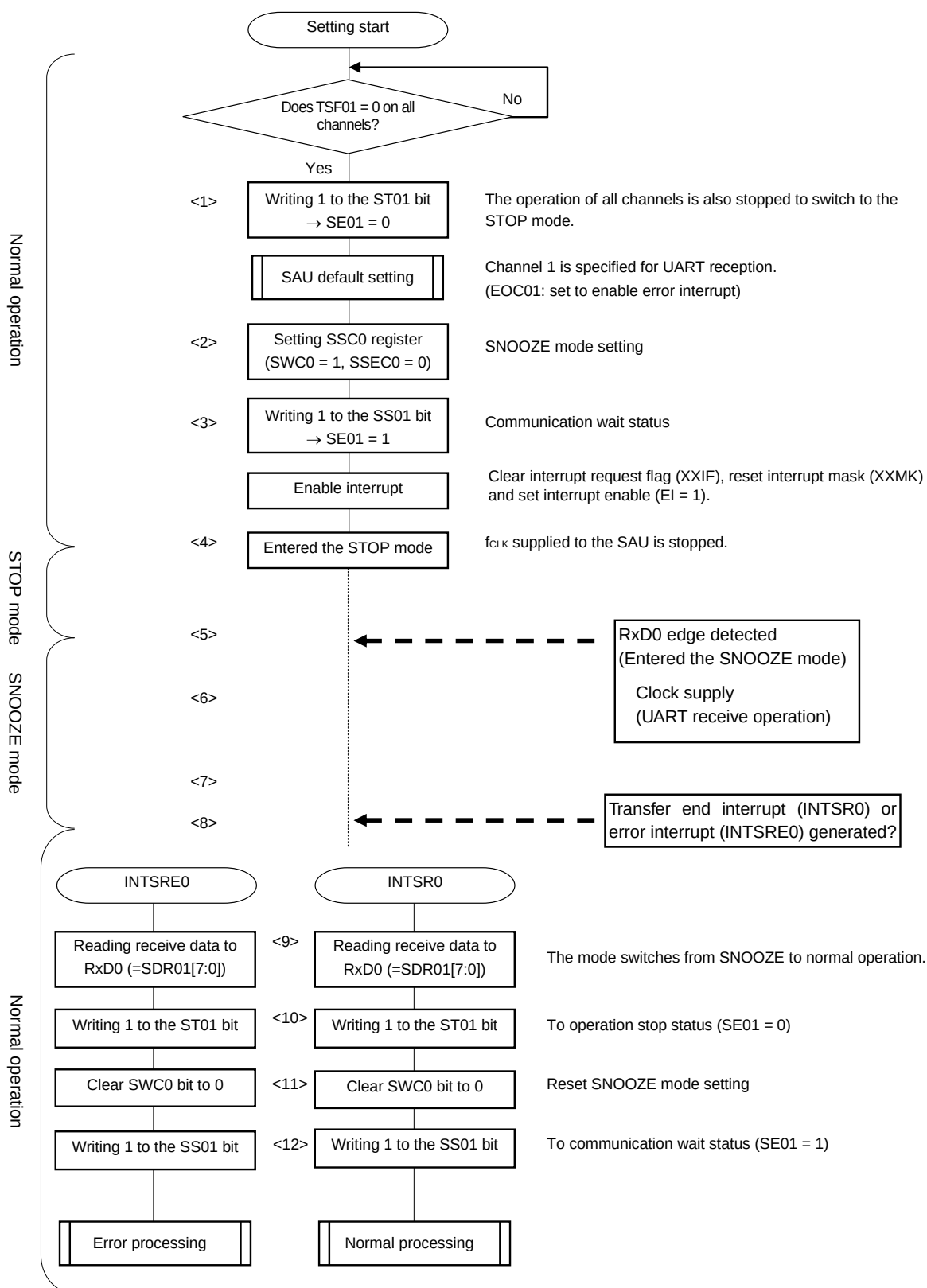
<R> Figure 11-93. Flowchart of SNOOZE Mode Operation (Normal Operation/Abnormal Operation <1>)
