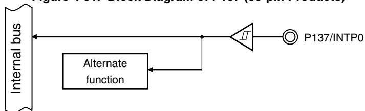
Figure 4-31. Block Diagram of P137 (30-pin Products)
