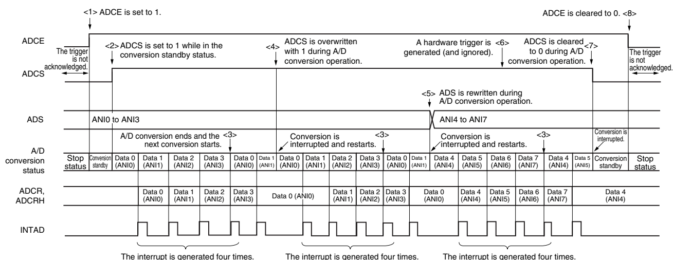
Figure 10-22. Example of Software Trigger Mode (Scan Mode, Sequential Conversion Mode) Operation Timing
