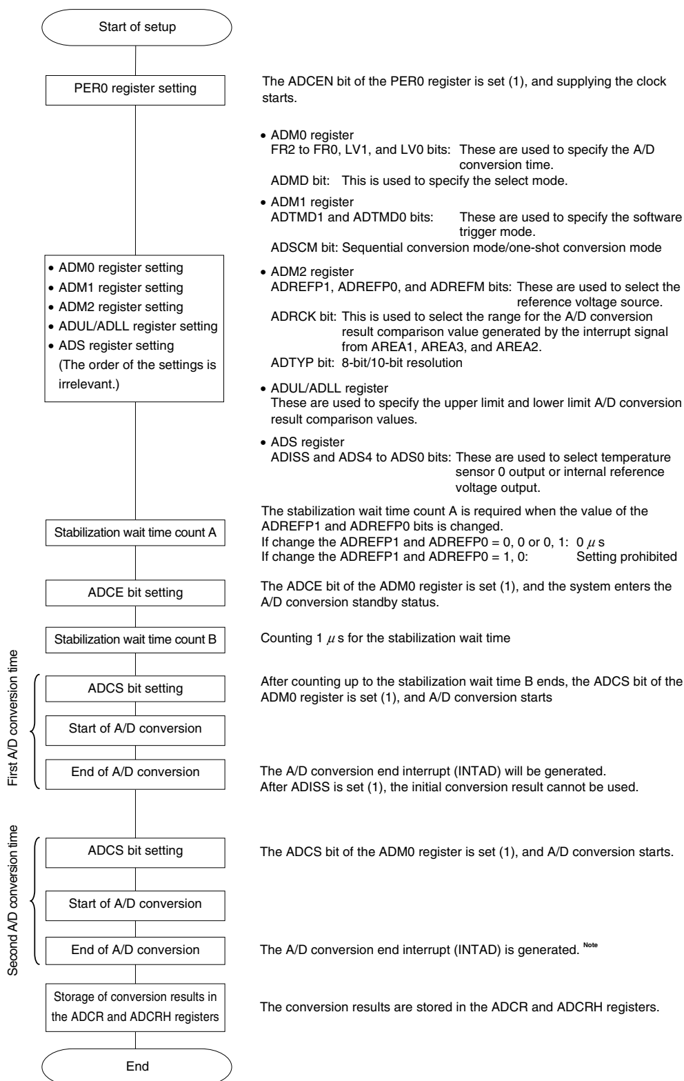
Figure 10-35. Setup When Using Temperature Sensor
