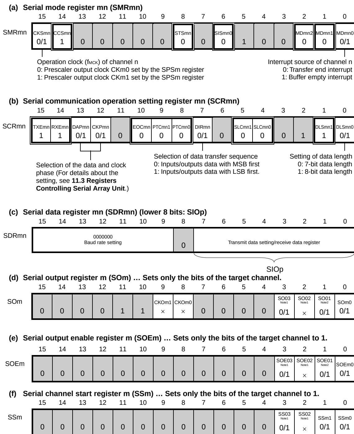
<R> Figure 11-64. Example of Contents of Registers for Slave Transmission/Reception of 3-Wire Serial I/O (CSI00, CSI01, CSI11, CSI20)
