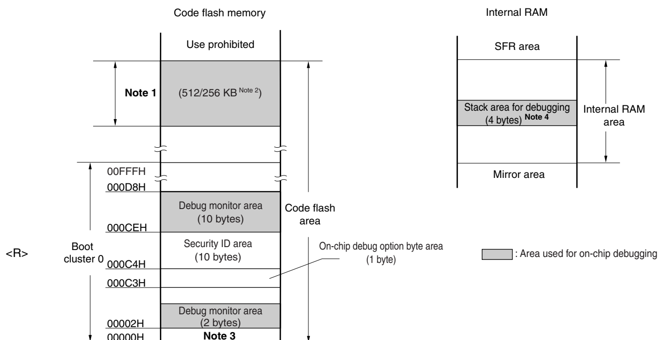
Figure 25-4. Memory Spaces Where Debug Monitor Programs Are Allocated
