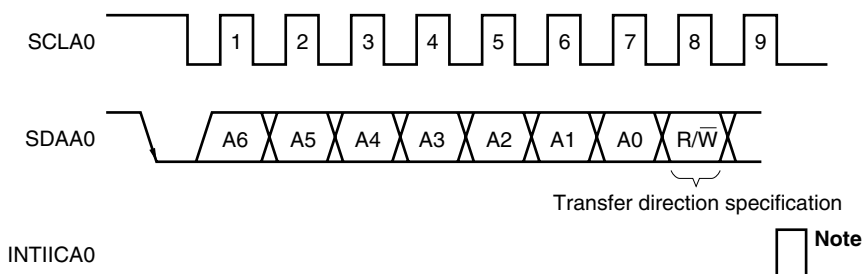
Figure 12-17. Transfer Direction Specification
