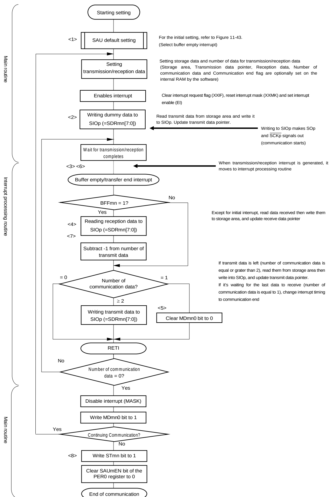
&lt;R&gt; Figure 11-49. Flowchart of Master Transmission/Reception (in Continuous Transmission/Reception Mode)
