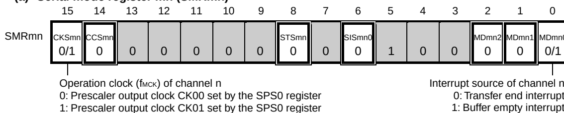
Figure 11-42. Example of Contents of Registers for Master Transmission/Reception of 3-Wire Serial I/O (CSI00, CSI01, CSI11, CSI20) (1/2)
