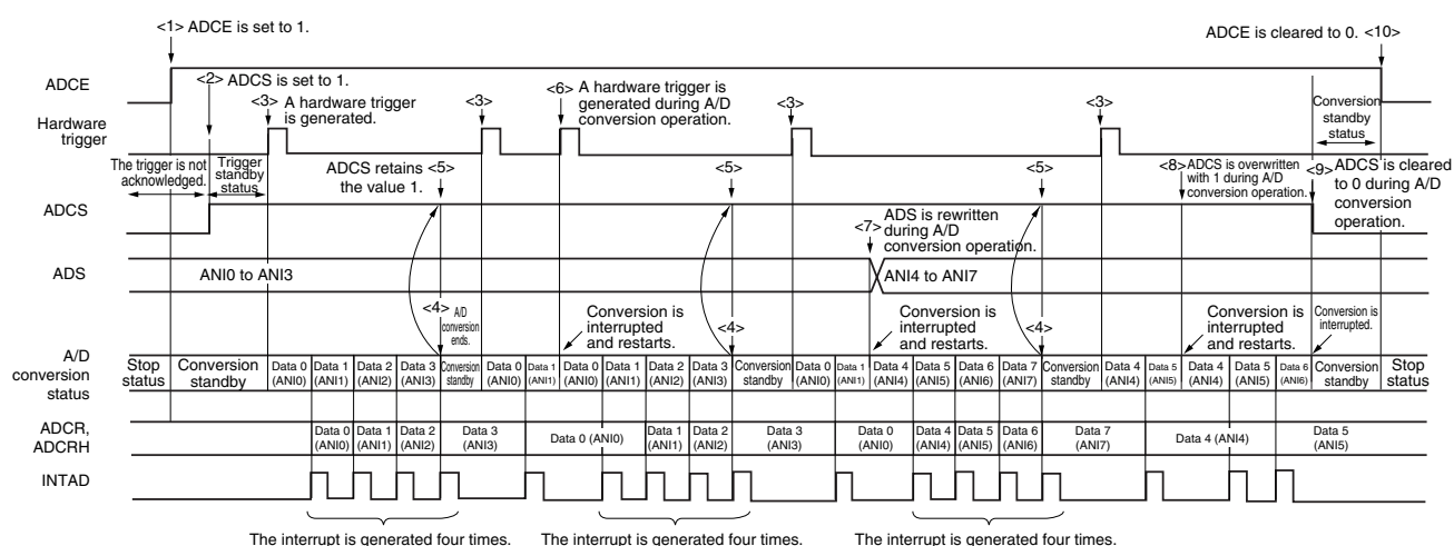
Figure 10-27. Example of Hardware Trigger No-Wait Mode (Scan Mode, One-Shot Conversion Mode) Operation Timing
