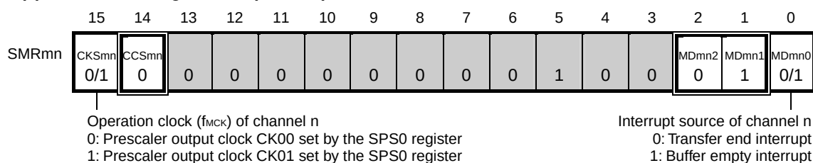
Figure 11-77. Example of Contents of Registers for UART Transmission (UART0 to UART2) (1/2)
