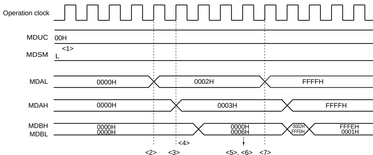
Figure 13-6. Timing Diagram of Multiplication (Unsigned) Operation ( 2 \times 3 = 6 )
