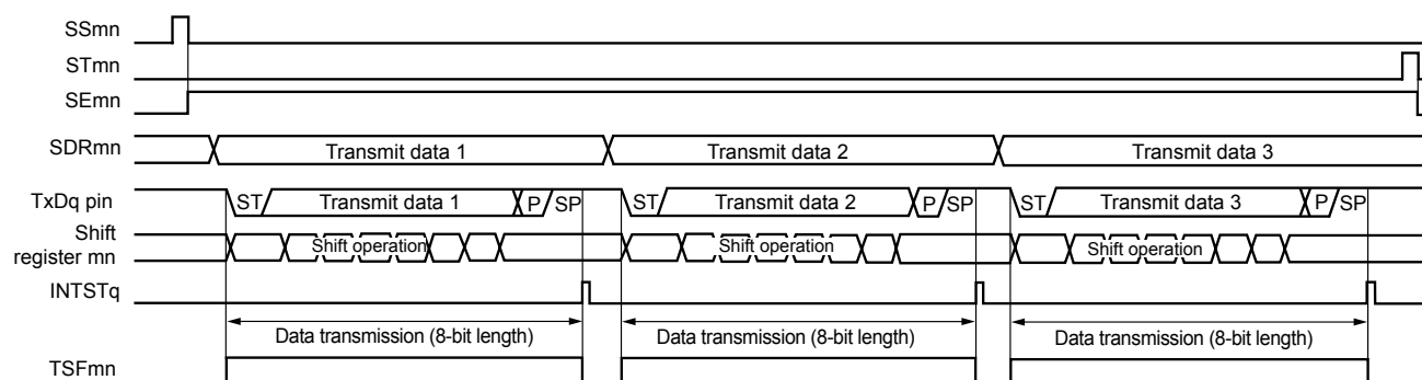
Figure 11-81. Timing Chart of UART Transmission (in Single-Transmission Mode)
