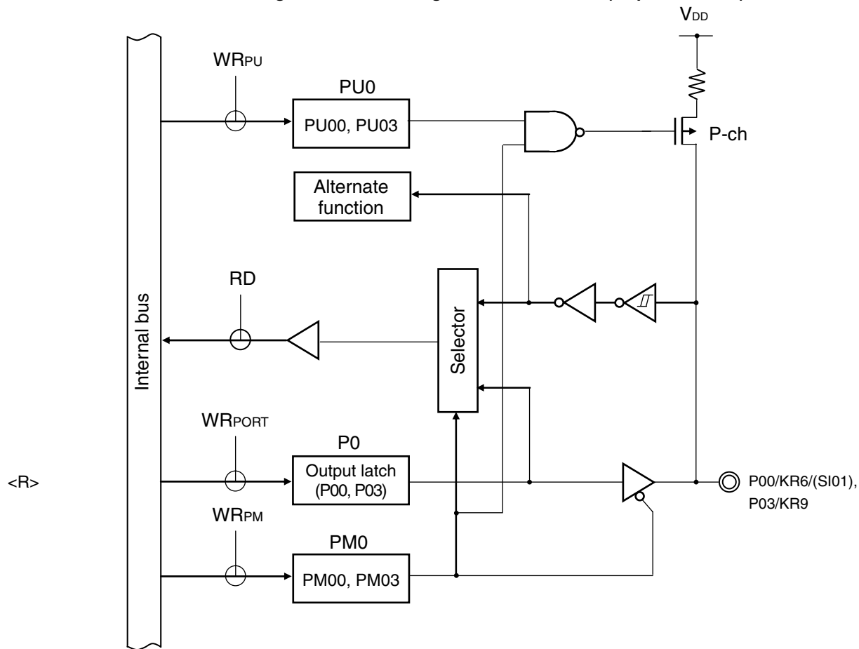
Figure 4-1. Block Diagram of P00, and P03 (24-pin Products)
