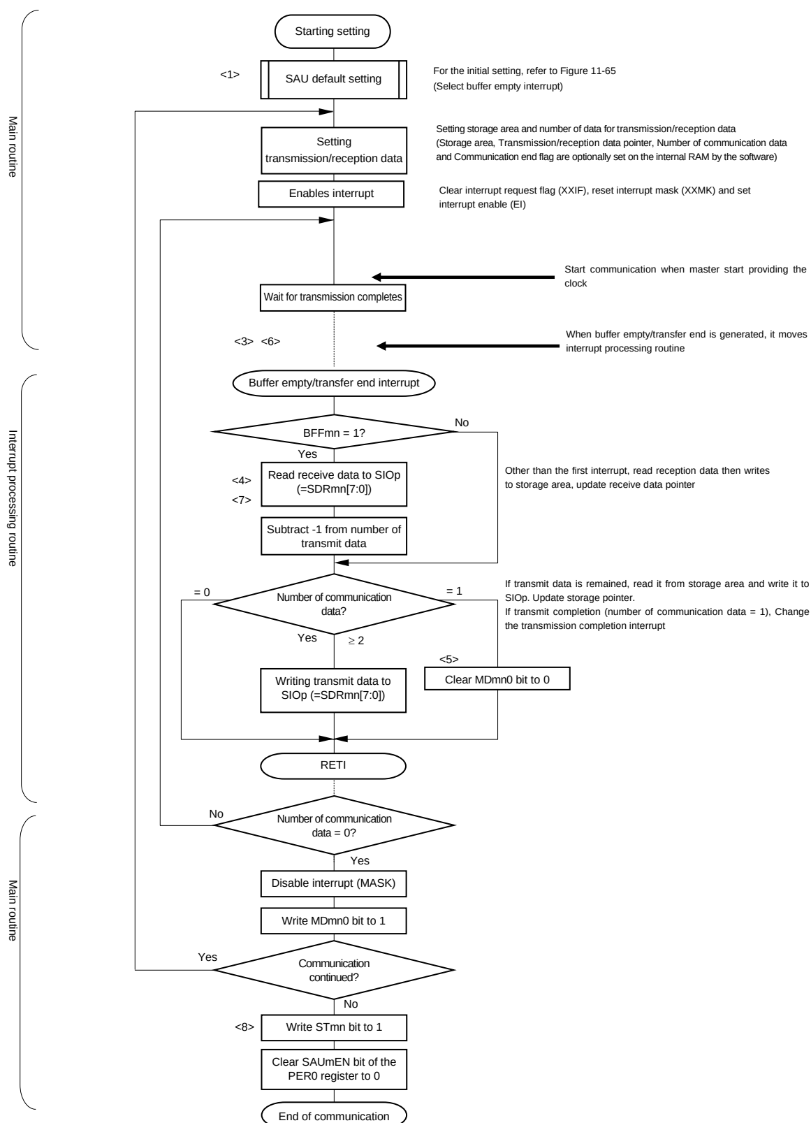
<R> Figure 11-71. Flowchart of Slave Transmission/Reception (in Continuous Transmission/Reception Mode)
