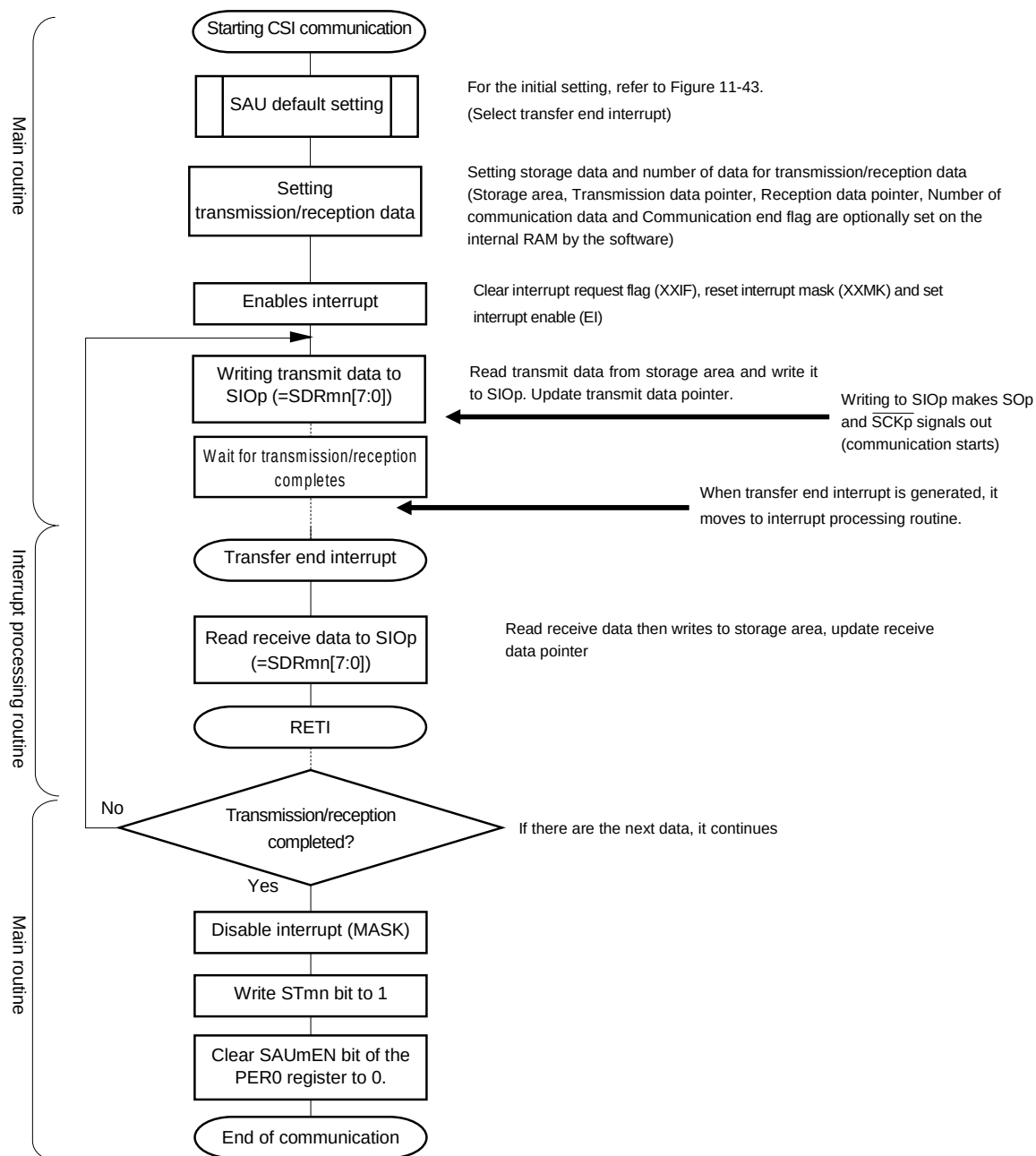
<R> Figure 11-47. Flowchart of Master Transmission/Reception (in Single-Transmission/Reception Mode)
