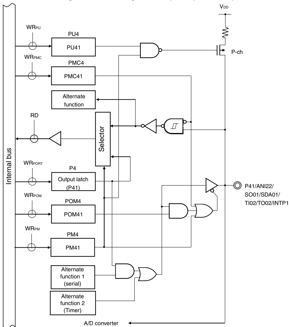
Figure 4-11. Block Diagram of P41 (20-, 24-pin Products)
