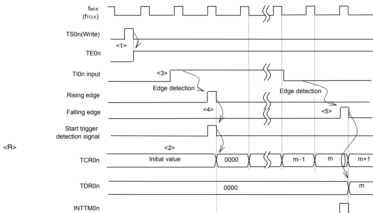
Figure 6-27. Operation Timing (In Capture & One-count Mode: High-level Width Measurement)
