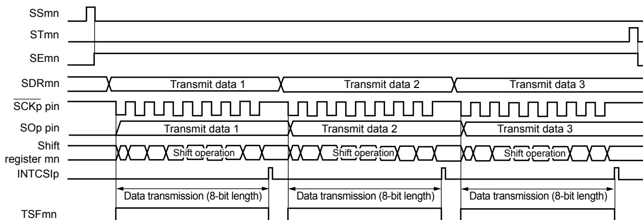
Figure 11-30. Timing Chart of Master Transmission (in Single-Transmission Mode) (Type 1: DAPmn = 0, CKPmn = 0)
