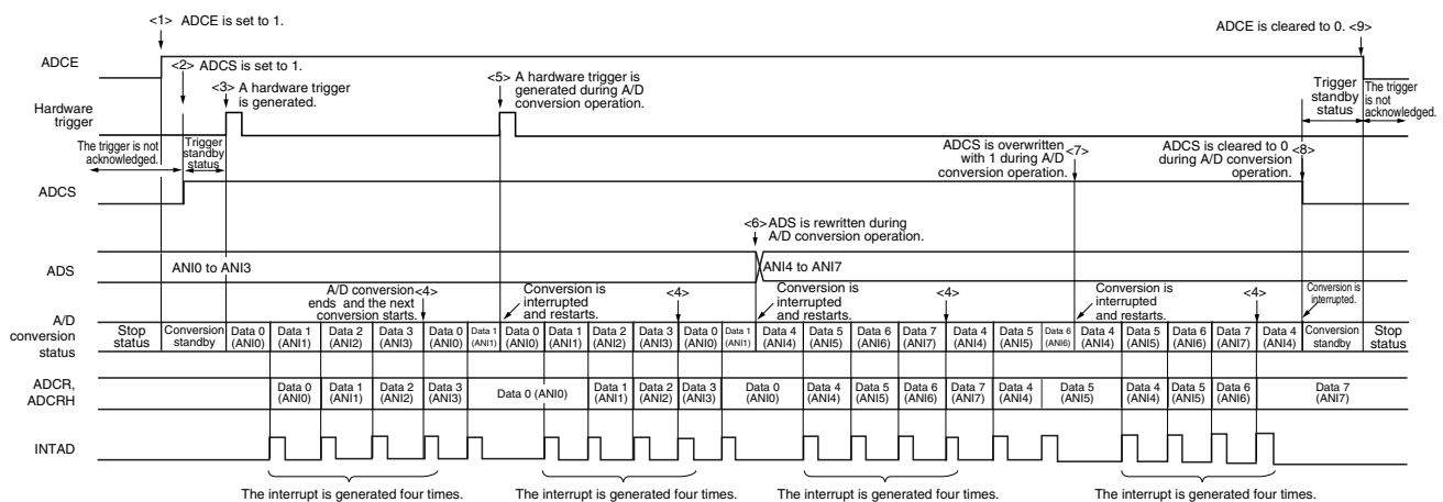
Figure 10-26. Example of Hardware Trigger No-Wait Mode (Scan Mode, Sequential Conversion Mode) Operation Timing
