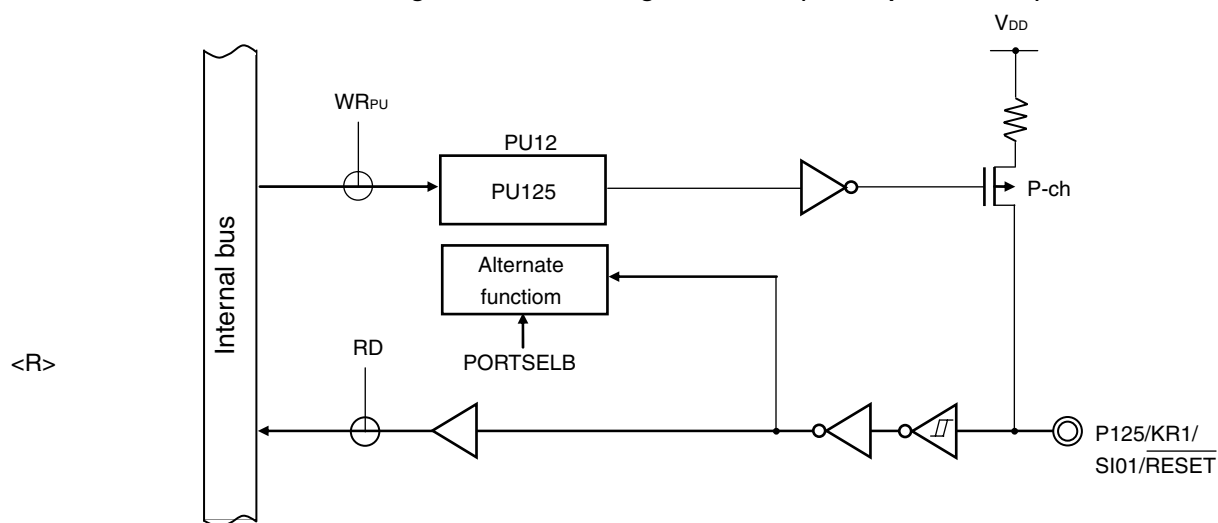
Figure 4-15 Block Diagram of P125 (20-, 24-pin Products)
