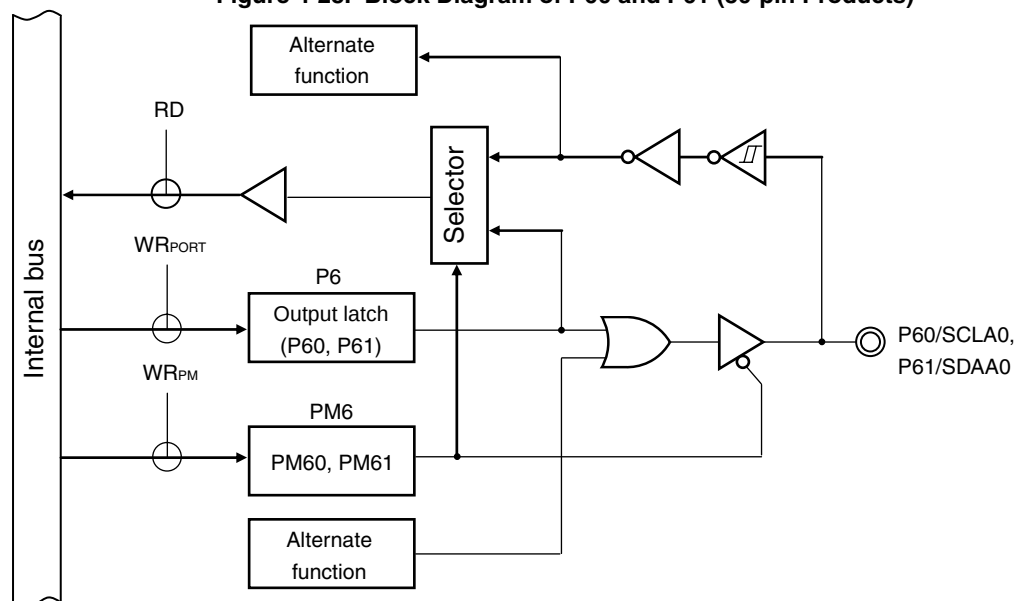
Figure 4-28. Block Diagram of P60 and P61 (30-pin Products)
