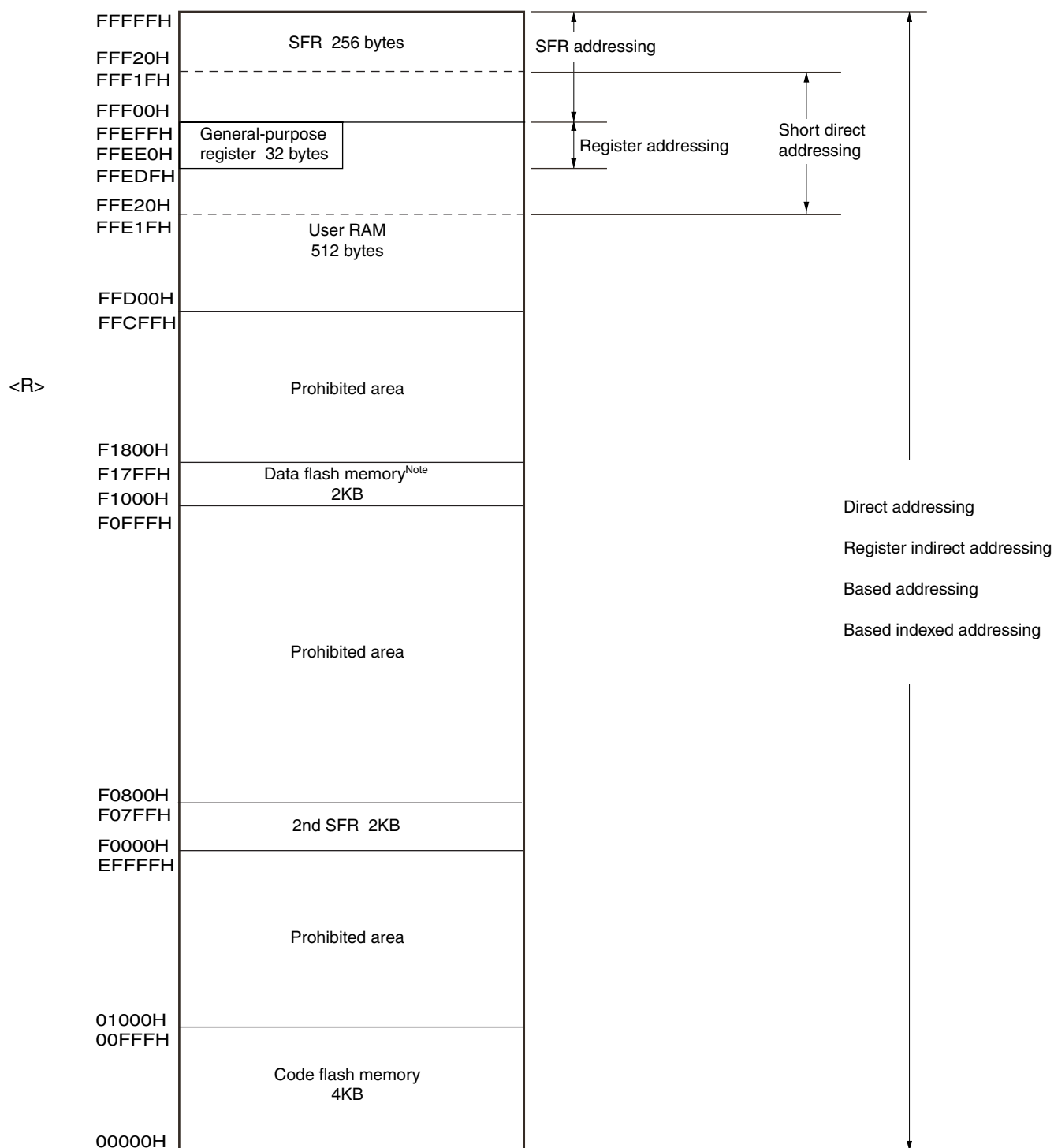
Figure 3-9. Correspondence Between Data Memory and Addressing for the R5F10x67, R5F10x77, R5F10xA7 (x = 2 or 3)
