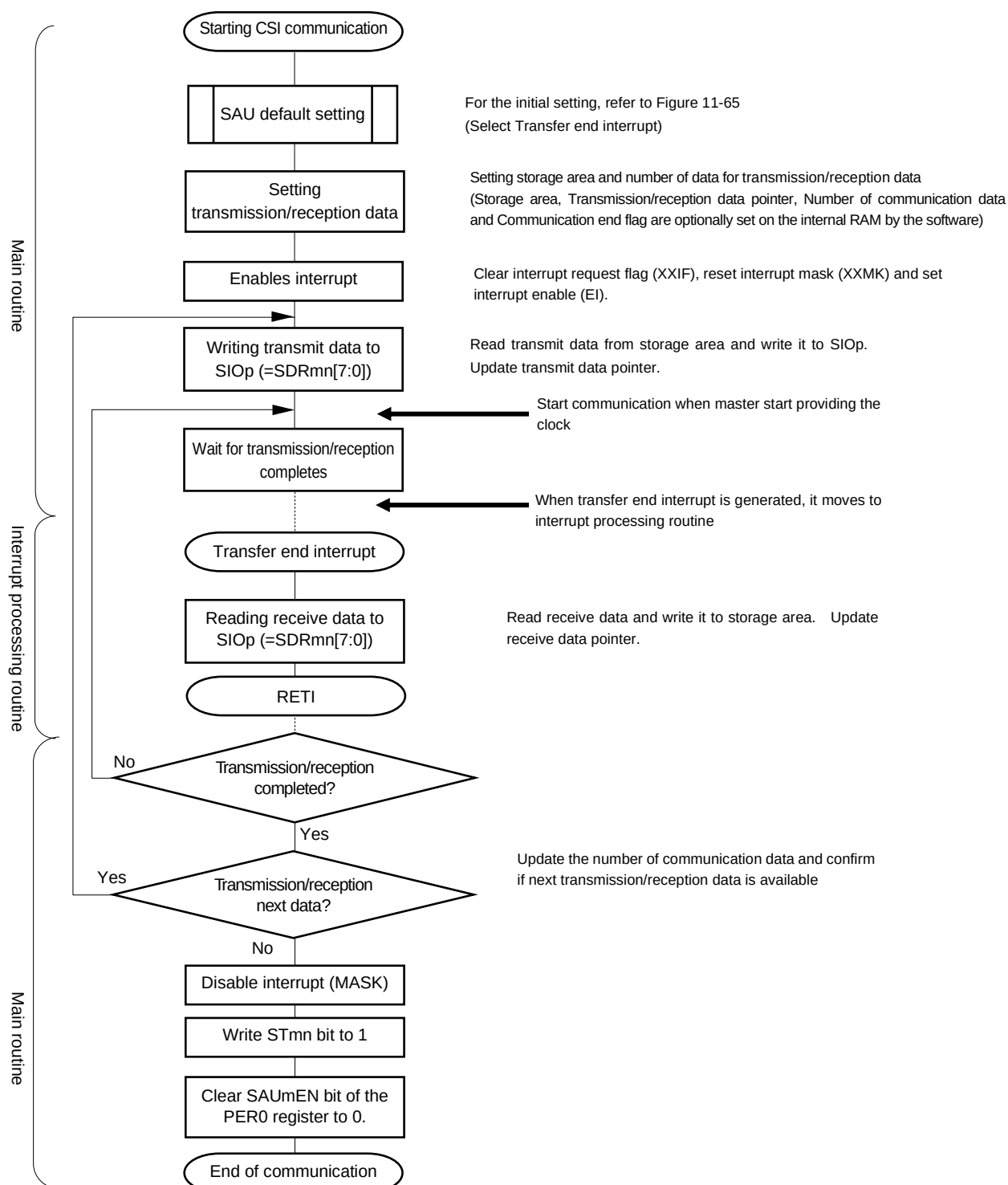
<R> Figure 11-69. Flowchart of Slave Transmission/Reception (in Single- Transmission/Reception Mode)
