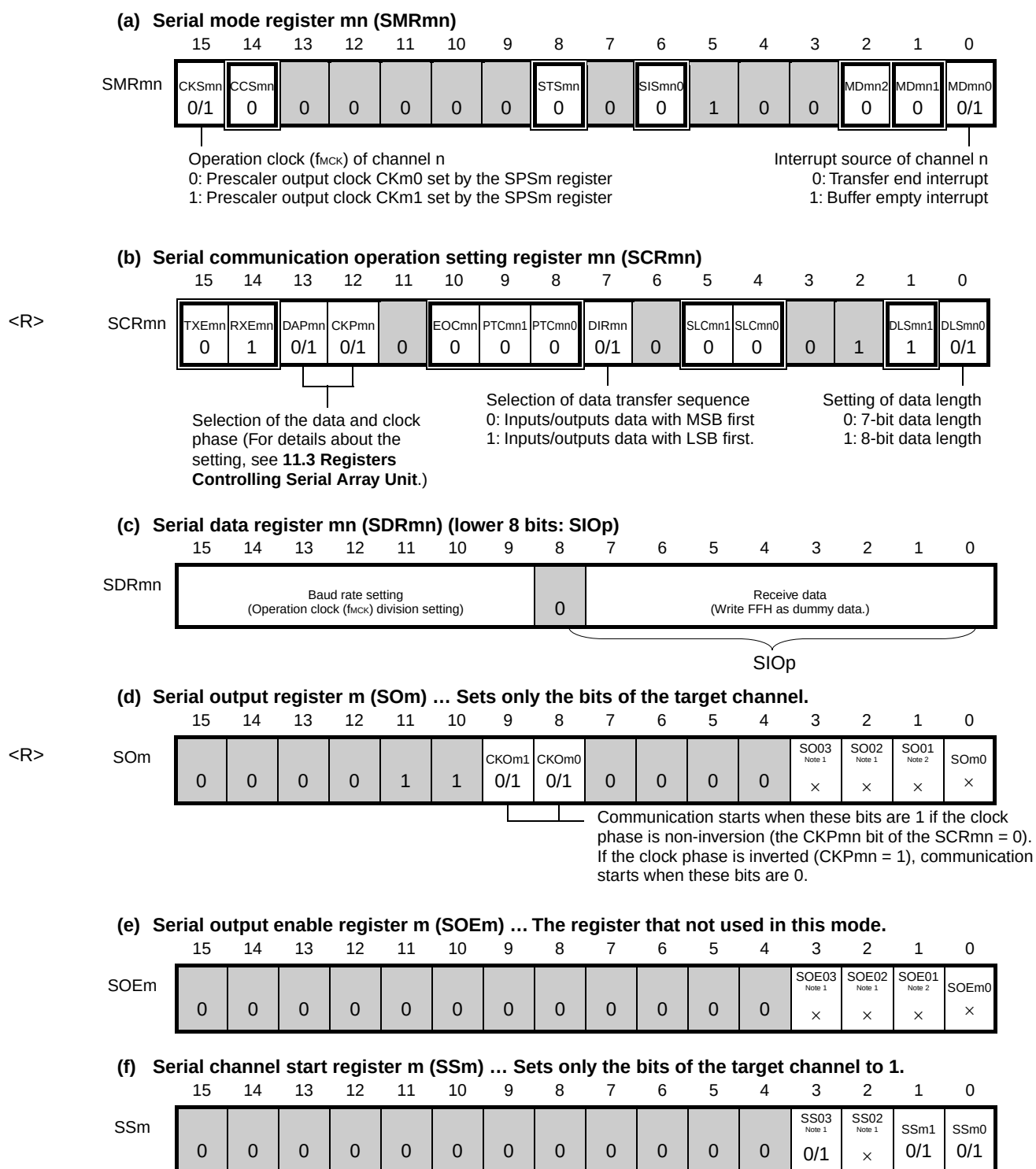
Figure 11-34. Example of Contents of Registers for Master Reception of 3-Wire Serial I/O (CSI00, CSI01, CSI11, CSI20)
