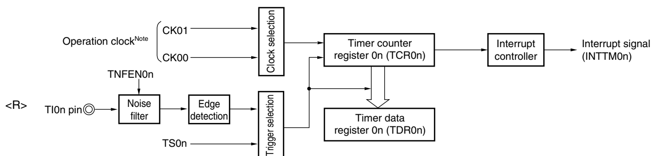
Figure 6-49. Block Diagram of Operation as Input Pulse Interval Measurement
