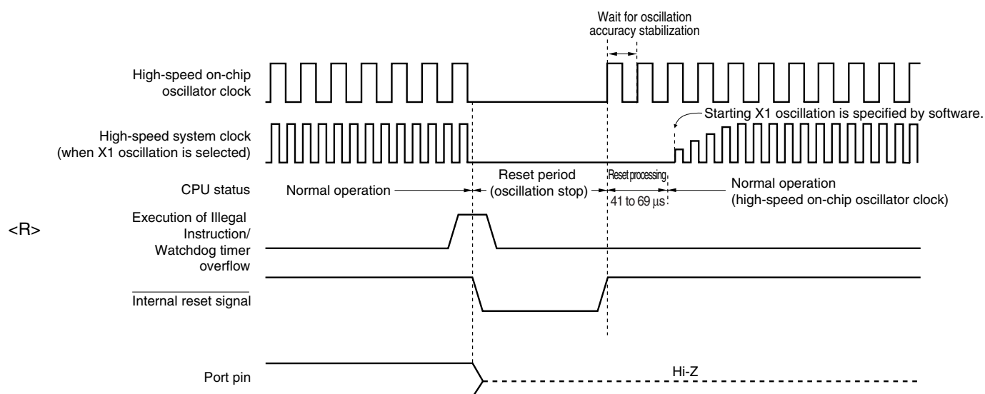
Figure 18-3. Timing of Reset Due to Execution of Illegal Instruction or Watchdog Timer Overflow
