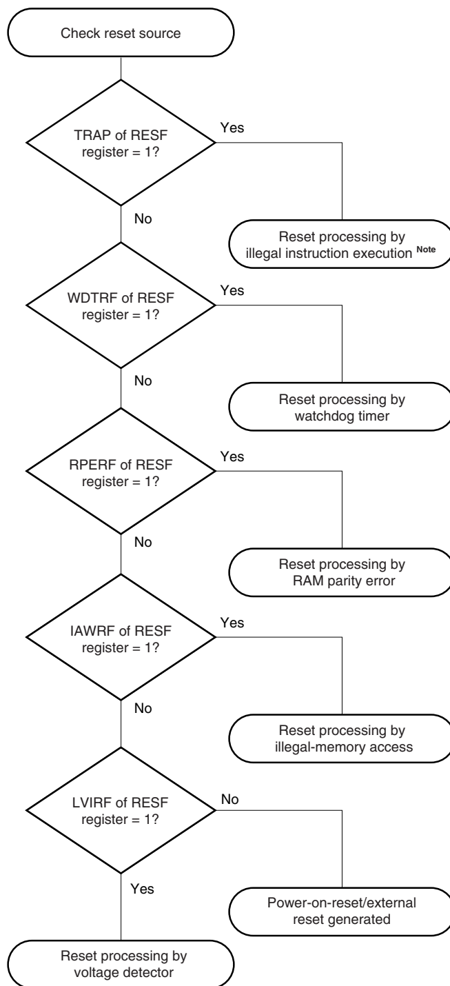
Figure 20-9. Checking reset source
