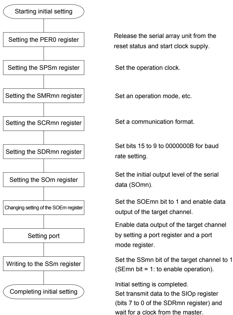
Figure 11-65. Initial Setting Procedure for Slave Transmission/Reception
