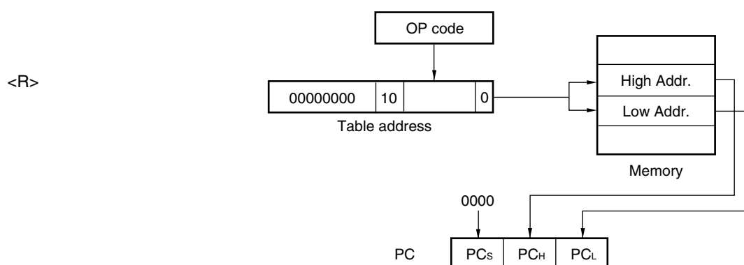
Figure 3-23. Outline of Table Indirect Addressing
