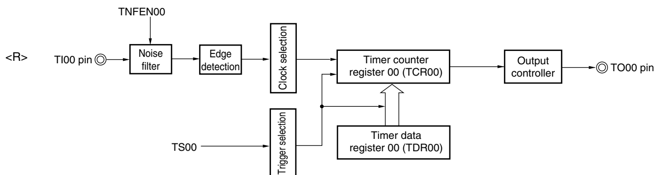
Figure 6-45. Block Diagram of Operation as Frequency Divider
