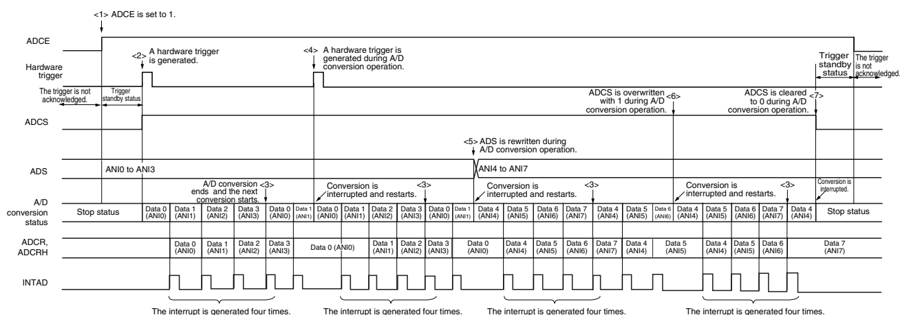
Figure 10-30. Example of Hardware Trigger Wait Mode (Scan Mode, Sequential Conversion Mode) Operation Timing
