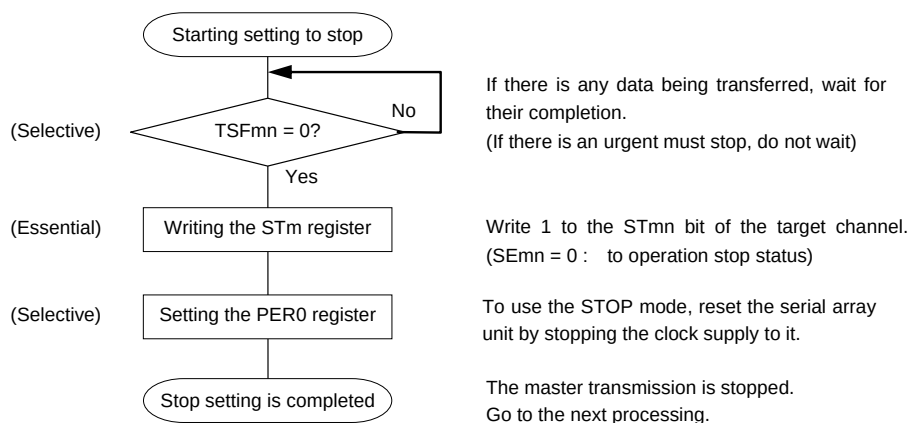
<R> Figure 11-87. Procedure for Stopping UART Reception
