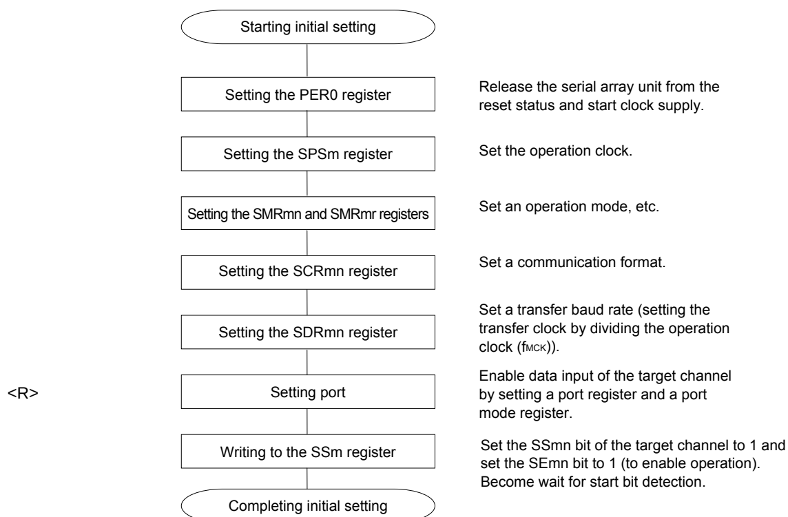
Figure 11-86. Initial Setting Procedure for UART Reception
