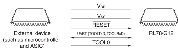
Figure 24-3. Environment for Writing Program to Flash Memory
