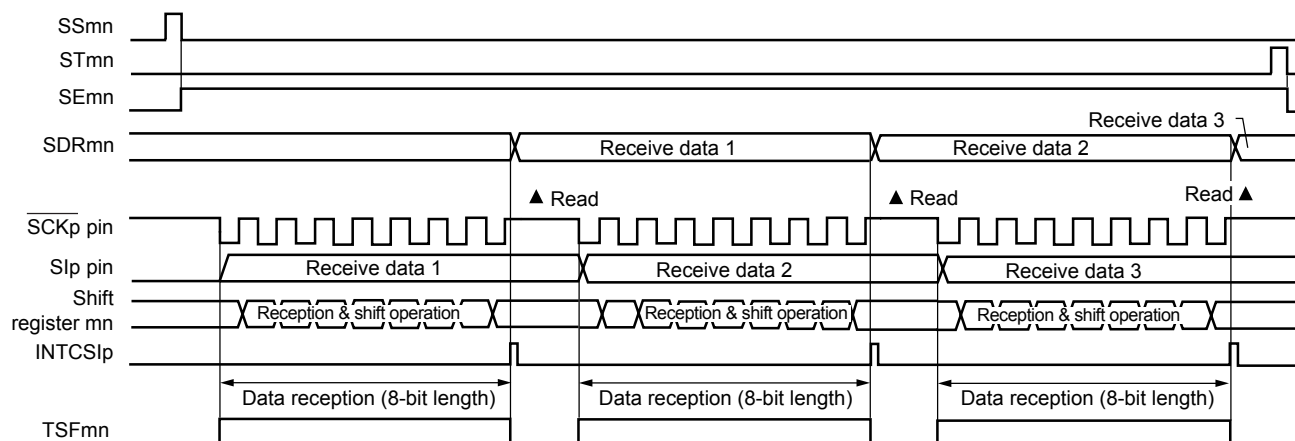
Figure 11-62. Timing Chart of Slave Reception (in Single-Reception Mode)
