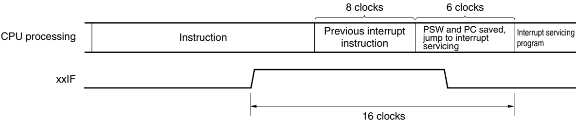
<R> Figure 15-12. Interrupt Request Acknowledgment Timing (Maximum Time)
