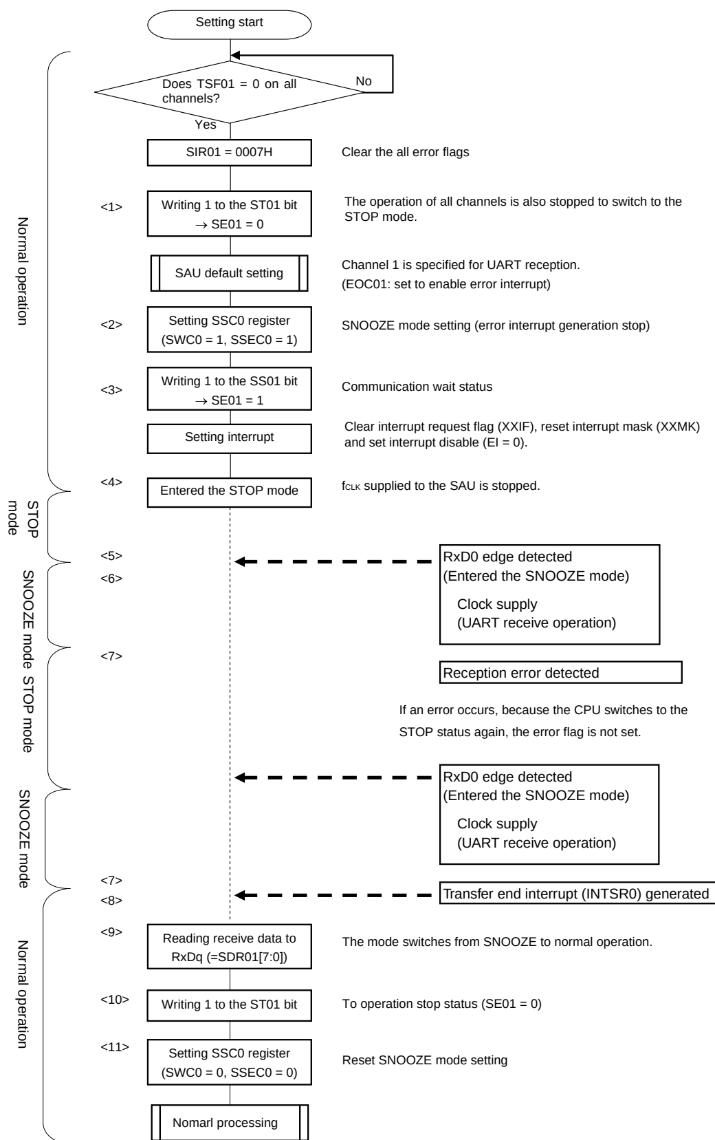
Figure 11-95. Flowchart of SNOOZE Mode Operation (Abnormal Operation &lt;2&gt;)
