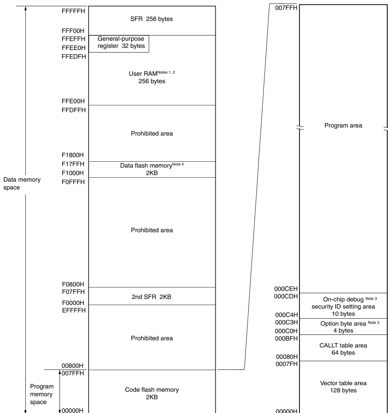
Figure 3-1. Memory Map for the R5F10266 and R5F10366
