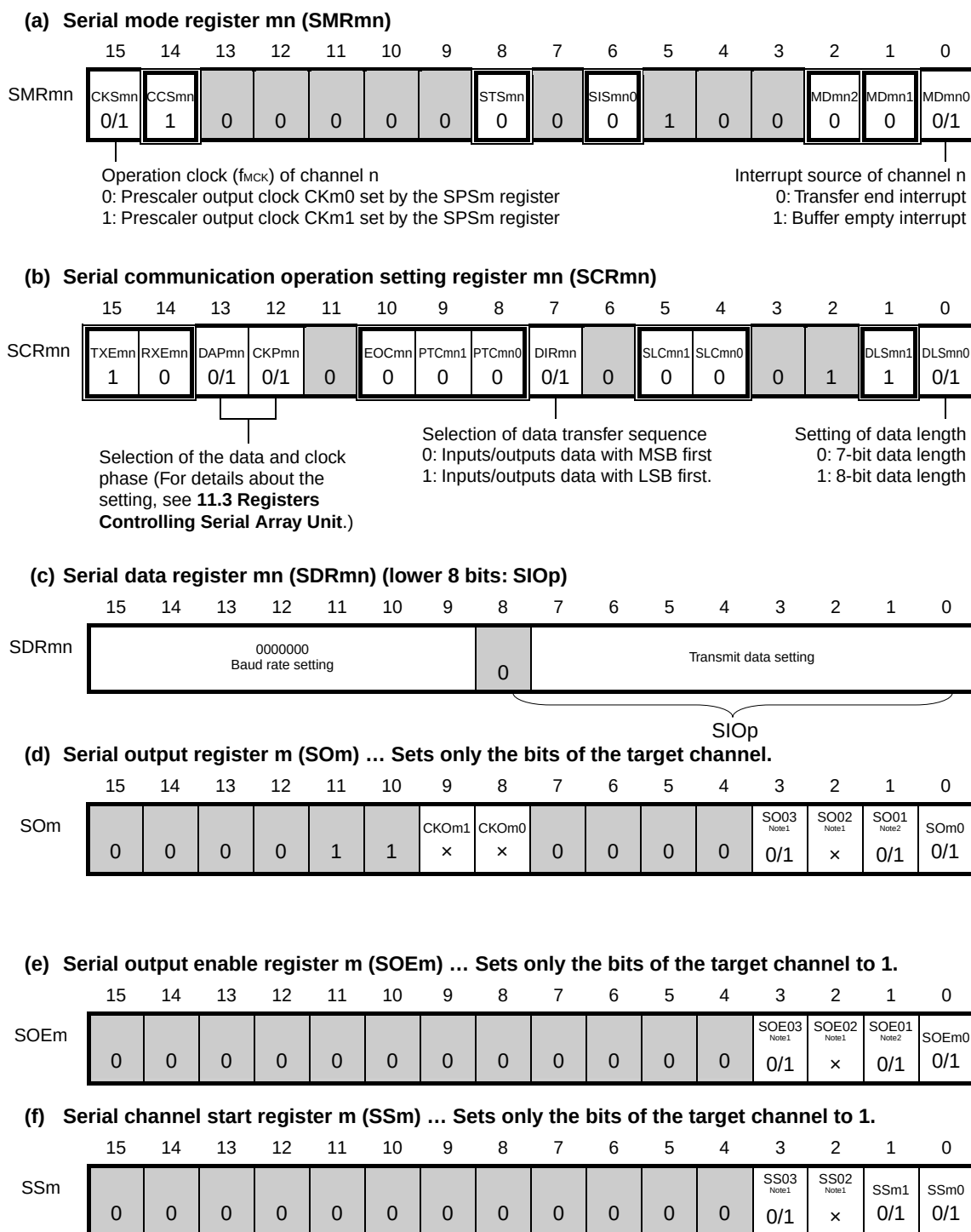
&lt;R&gt; Figure 11-50. Example of Contents of Registers for Slave Transmission of 3-Wire Serial I/O (CSI00, CSI01, CSI11, CSI20)
