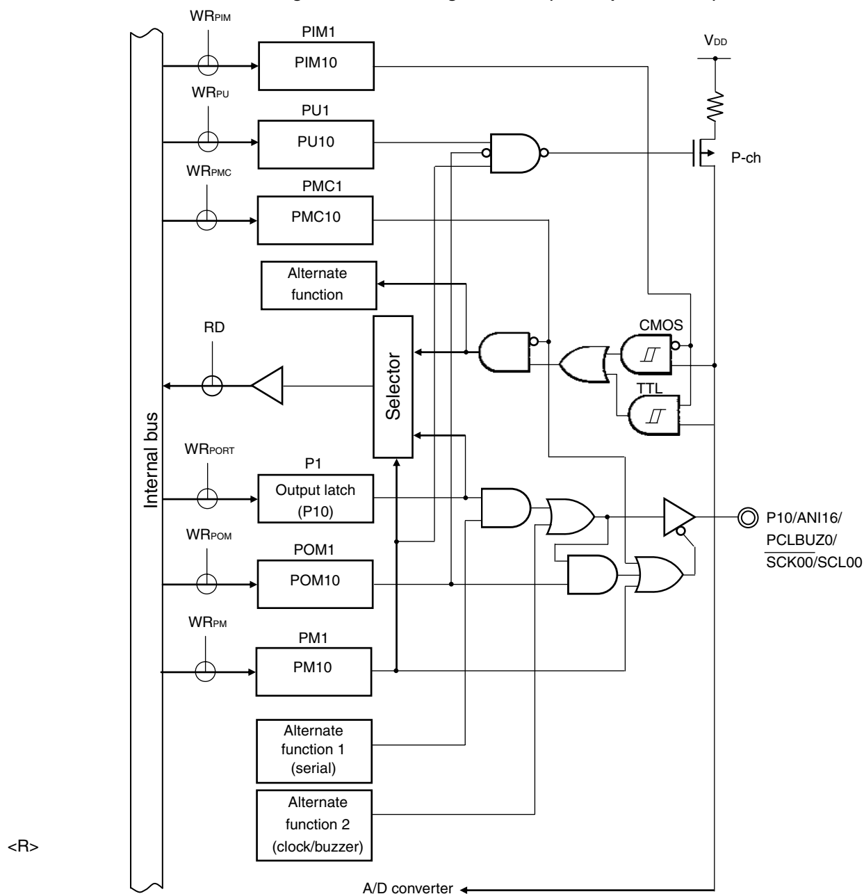
Figure 4-4. Block Diagram of P10 (20-, 24-pin Products)
