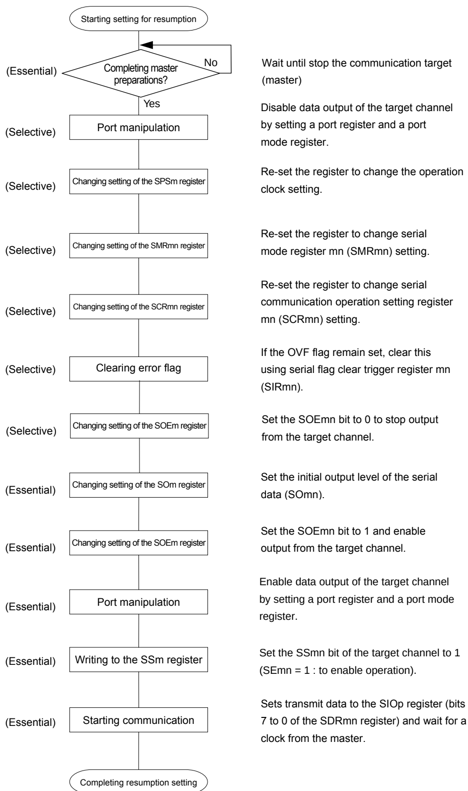
Figure 11-53. Procedure for Resuming Slave Transmission
