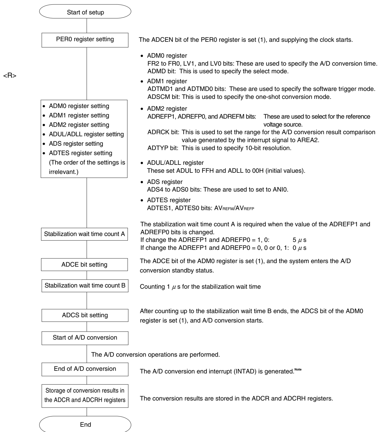
Figure 10-36. Setting up Test Trigger Mode
