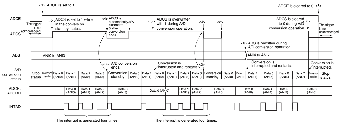
Figure 10-23. Example of Software Trigger Mode (Scan Mode, One-Shot Conversion Mode) Operation Timing
