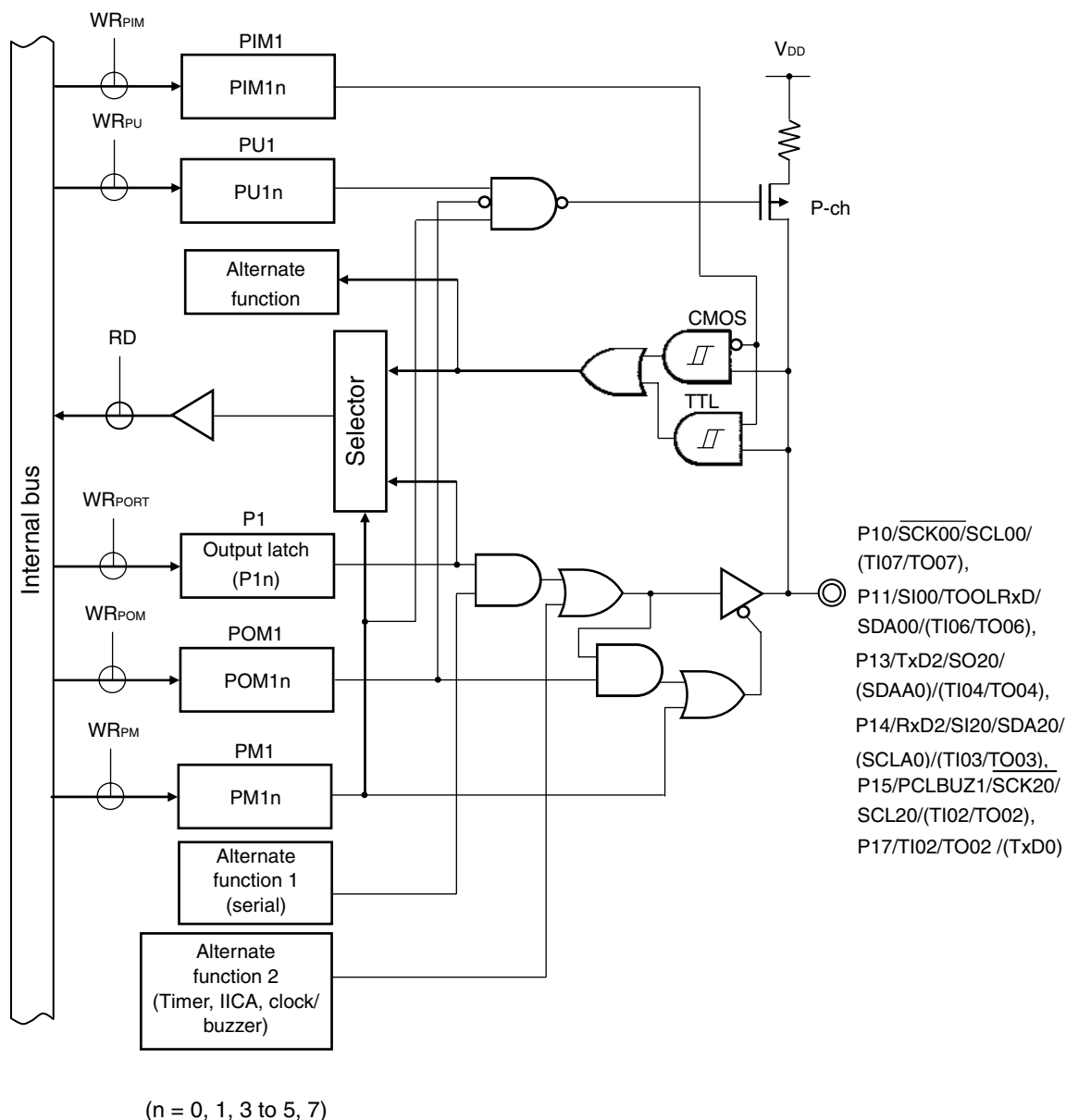
Figure 4-19. Block Diagram of P10, P11, P13 to P15, P17 (30-pin Products)
