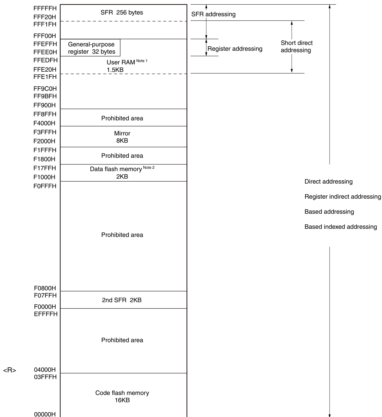
Figure 3-12. Correspondence Between Data Memory and Addressing for the R5F10x6A, and R5F10x7A (x = 2 or 3)
