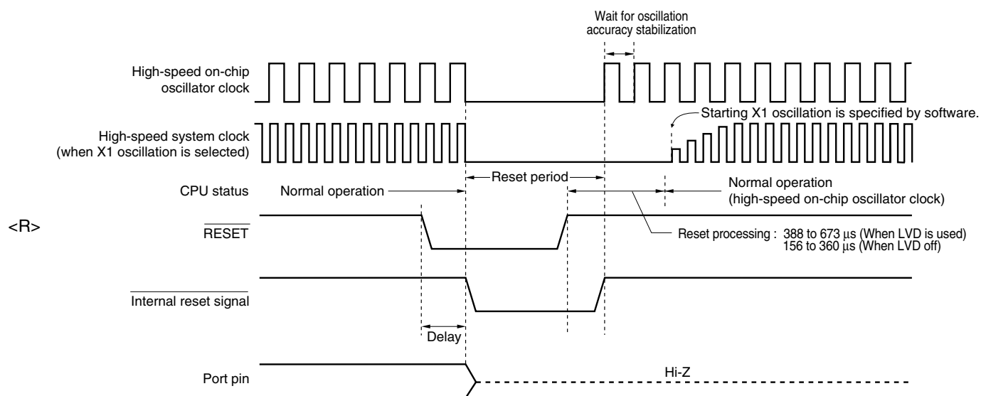
Figure 18-2. Timing of Reset by \overline{\text{RESET}} Input
