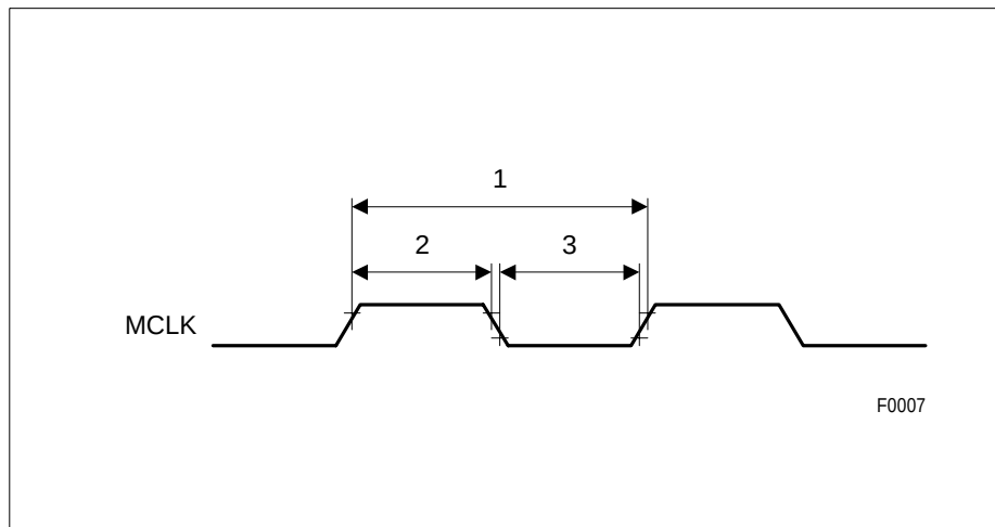
Figure 79 MCLK Timing
