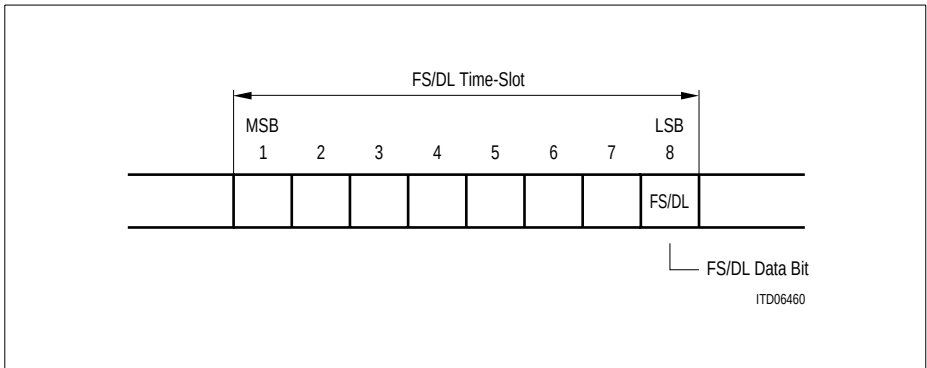
Figure 59 Receive FS/DL-Bits in Time Slot 0 on RDO (T1/J1)
