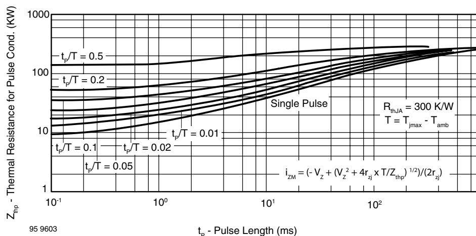
Figure 11. Thermal Response
