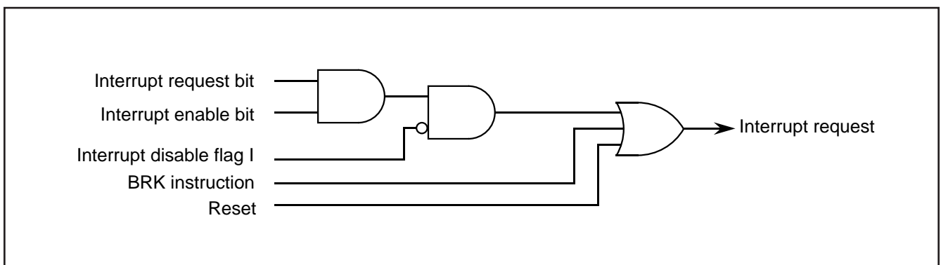
Fig. 5 Interrupt control
