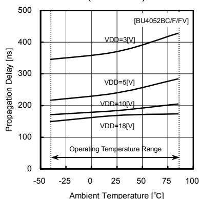
Fig.23 propagation delay time tPHZ (CONT—OUT)
