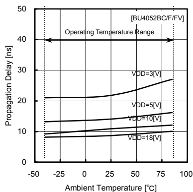
Fig.20 propagation delay time tPLH (IN—OUT)
