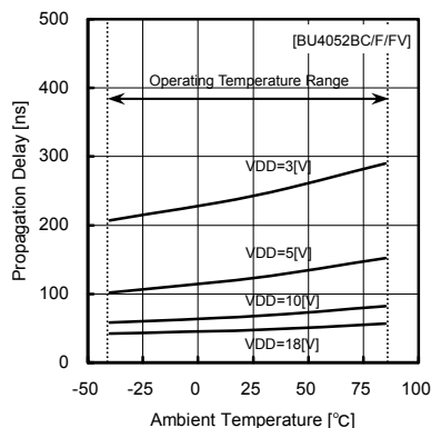
Fig.29 propagation delay time tPLZ (INH—OUT)
