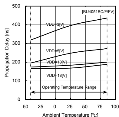
Fig.16 propagation delay time tPHZ (INH – OUT)
