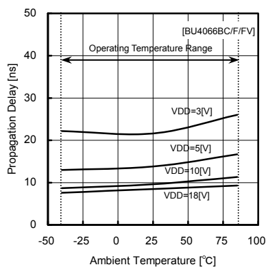
Fig.2 rising propagation delay (IN—OUT)
