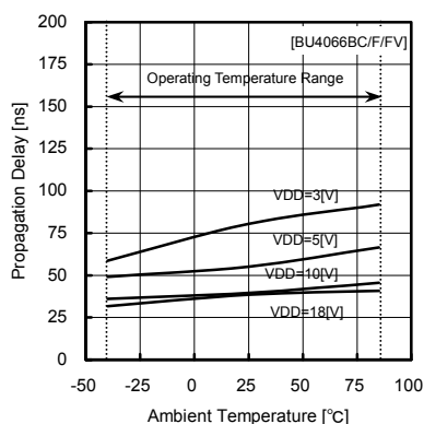
Fig.5 falling propagation delay (CONT—OUT, tPHZ)
