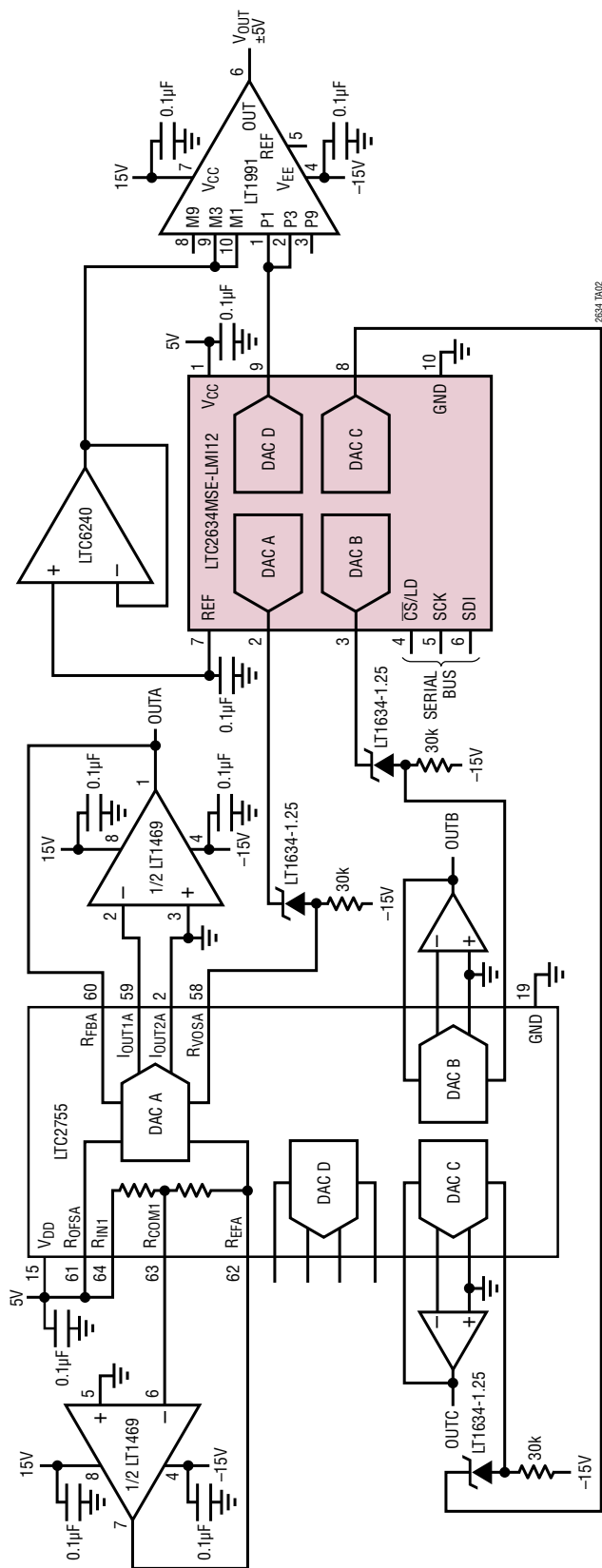
LTC2634 DACs Adjusts LTC2755-16 Offsets, Amplified with LT ® 1991 PGA to \pm 5V
