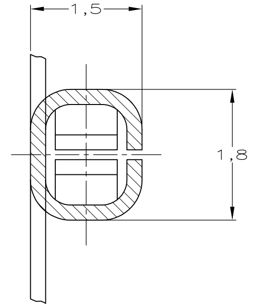
SECTION B-B SCALE 20:1
