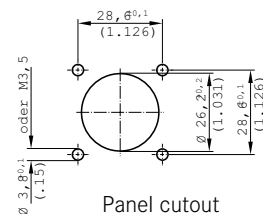
Panel cutout
