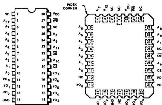
DUAL-IN-LINE TOP VIEW
