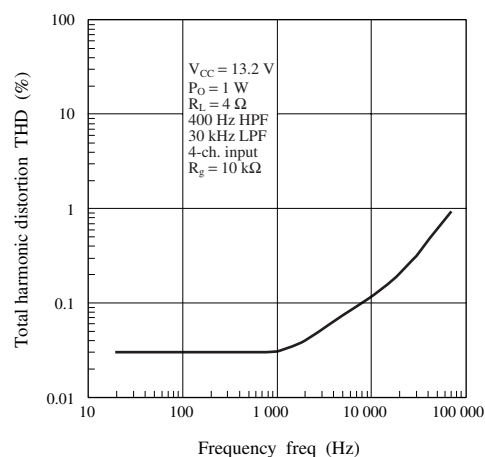
THD — freq
