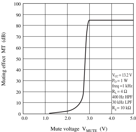
MT — V_{\text{MUTE}}
