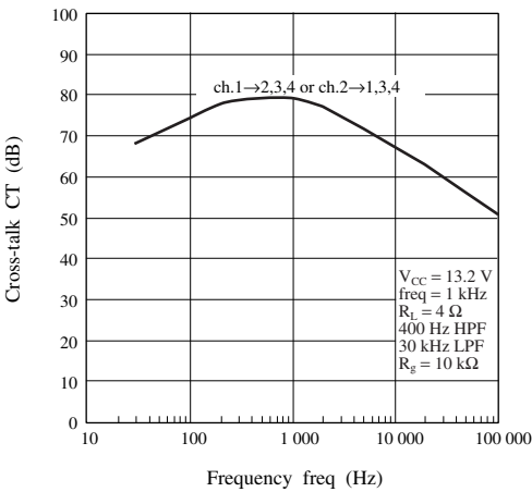
CT — freq
