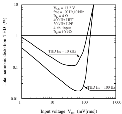
THD — V_{IN}
