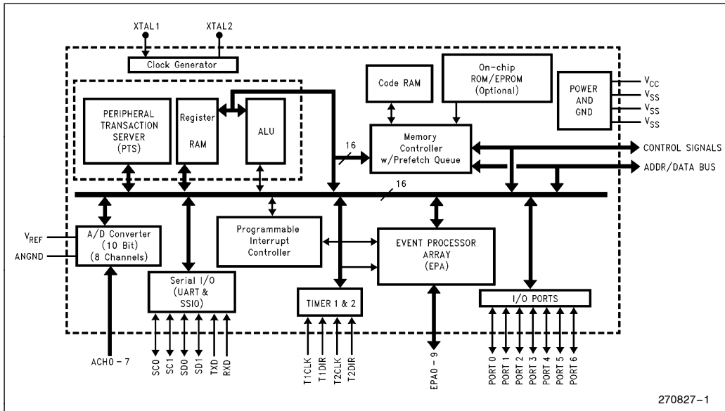
Figure 1. Block Diagram
