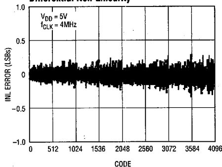
Differential Non-Linearity
