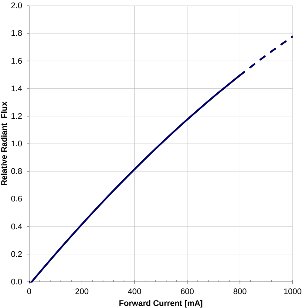
Relative Radiant Flux vs. Forward Current:
