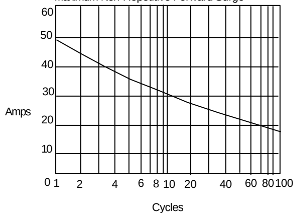
Figure 4 Maximum Non-Repetitive Forward Surge
