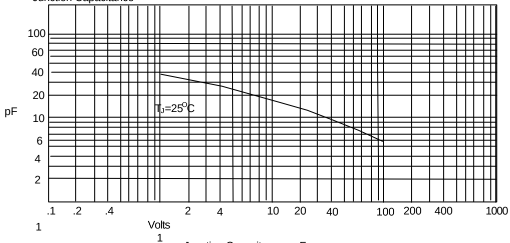
Figure 3 Junction Capacitance
