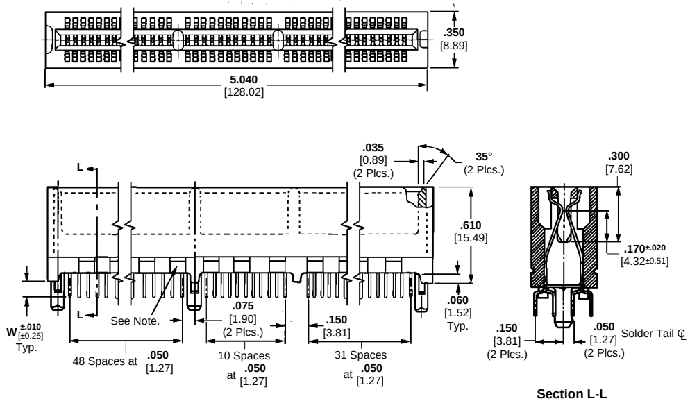
Section L-L
