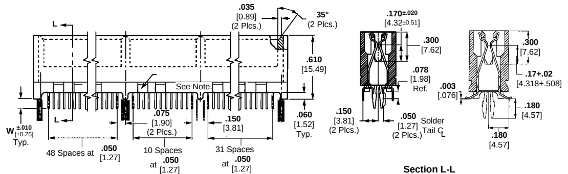
Section L-L
