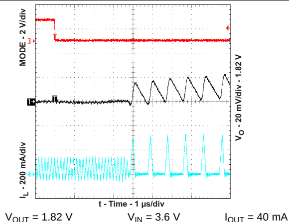
Figure 33. Power-Save Mode Operation
