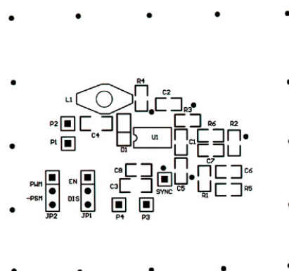
FIGURE 10. Boost—Top Silk Screen
