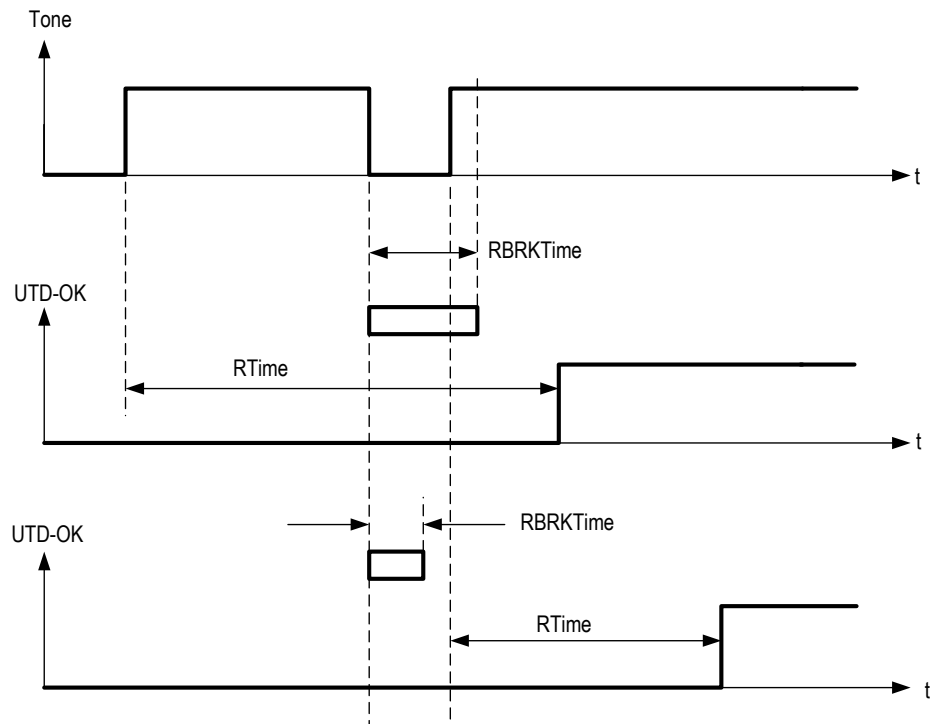
Figure - 17 Example of UTD Recognition Timing
