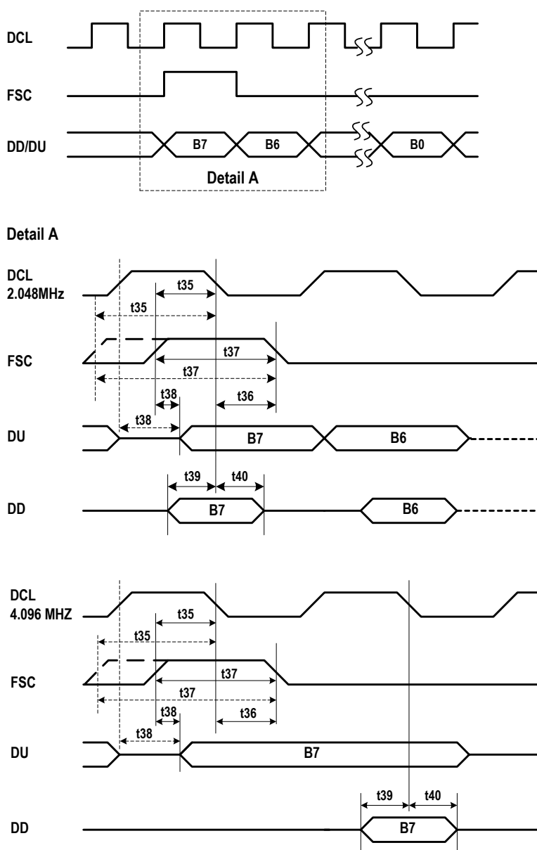
Figure - 47 GCI Interface Timing
