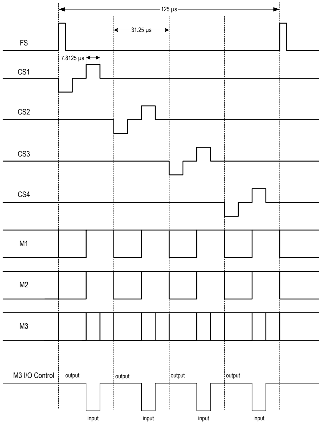
Figure - 38 RSLIC Control Timing Diagram
