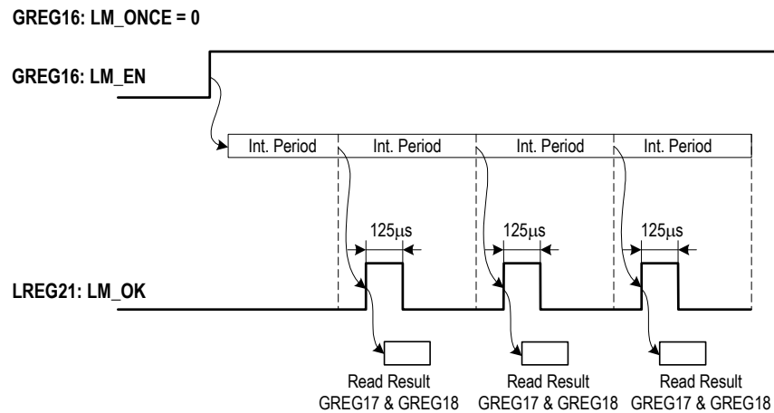
Figure - 21 Continuous Measurement Sequence (AC & DC Level Meter)
