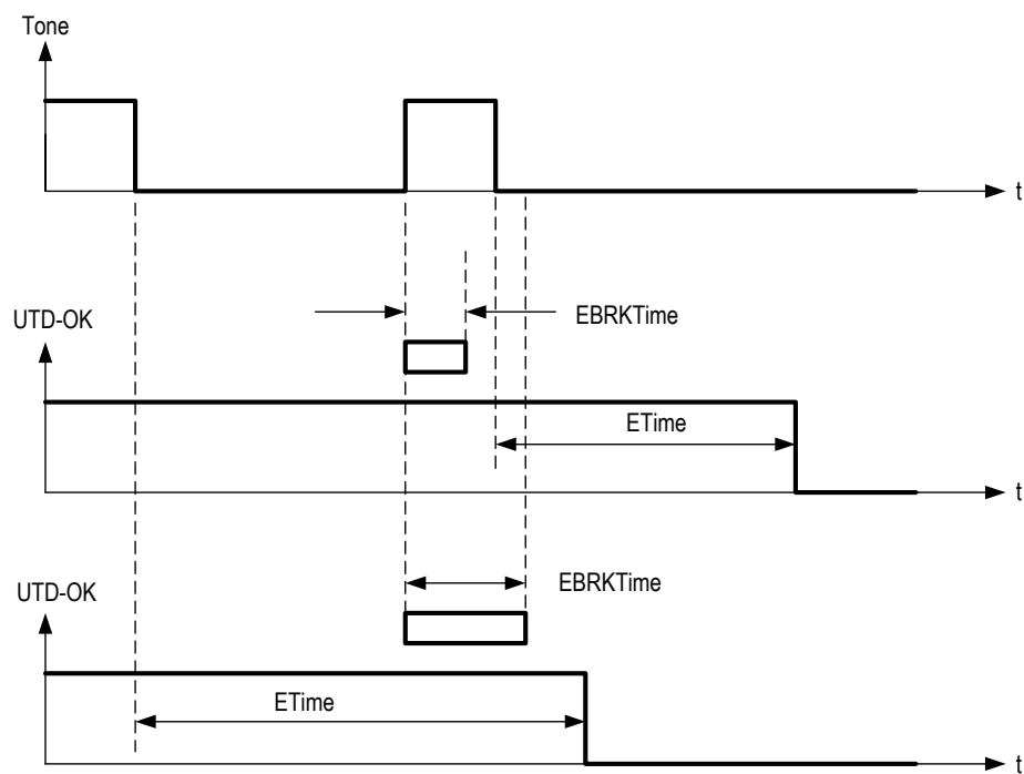
Figure - 18 Example of UTD Tone End Detection Timing
