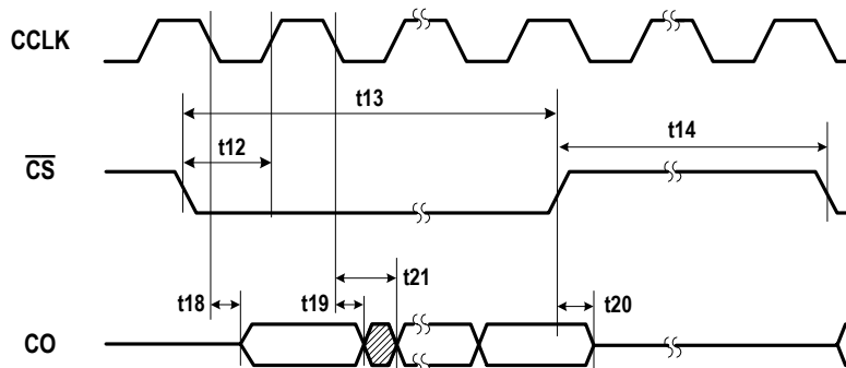
Figure - 44 MPI Output Timing
