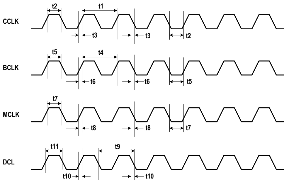
Figure - 42 Clock Timing
