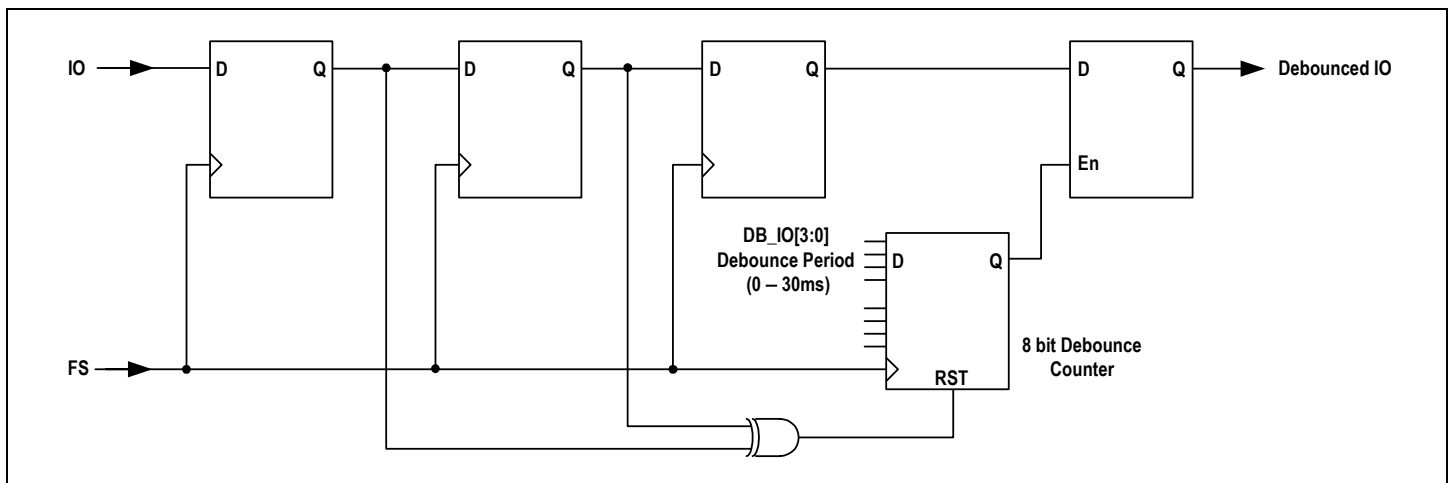
Figure - 40 IO Debounce Filter
