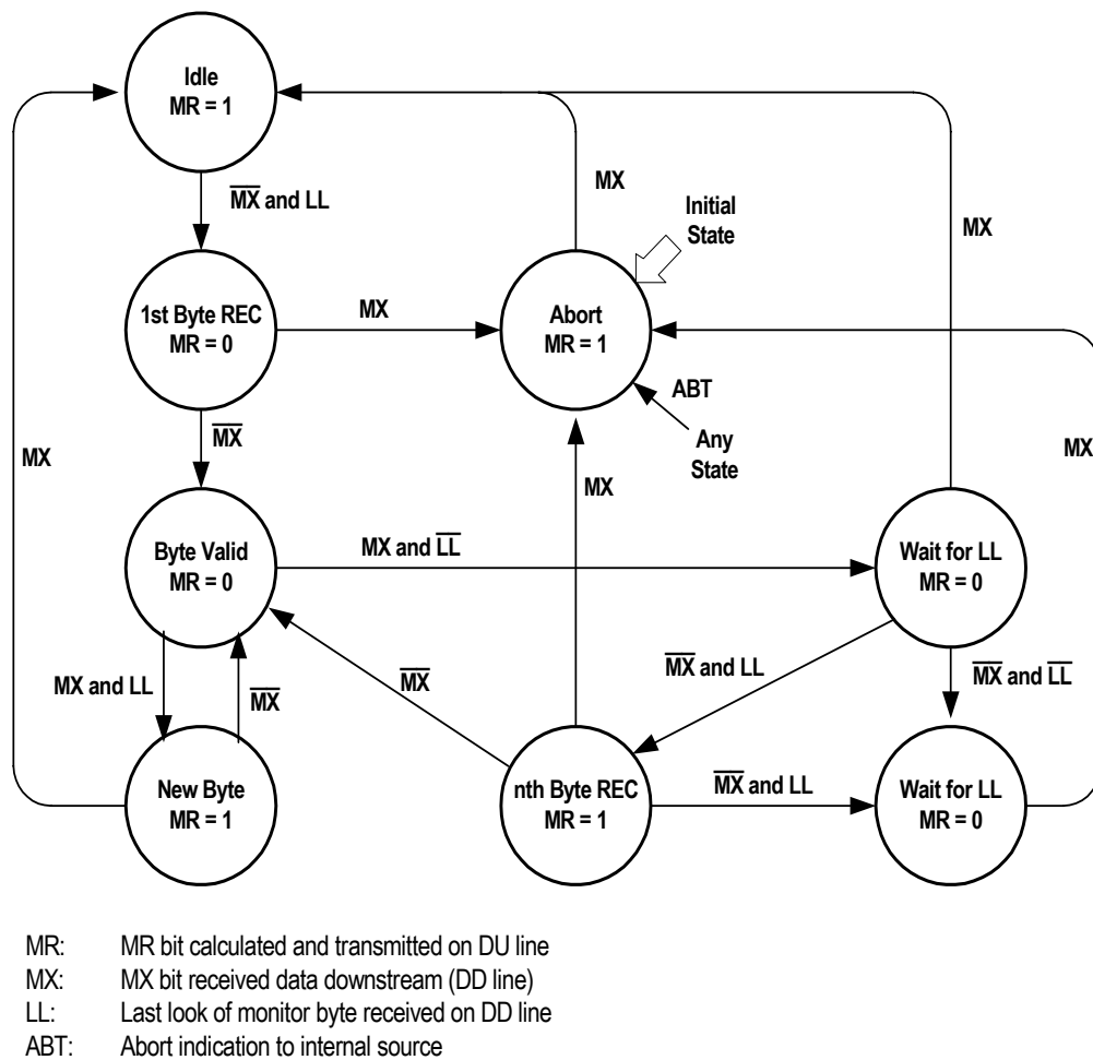
Figure - 34 State Diagram of the Monitor Receiver
