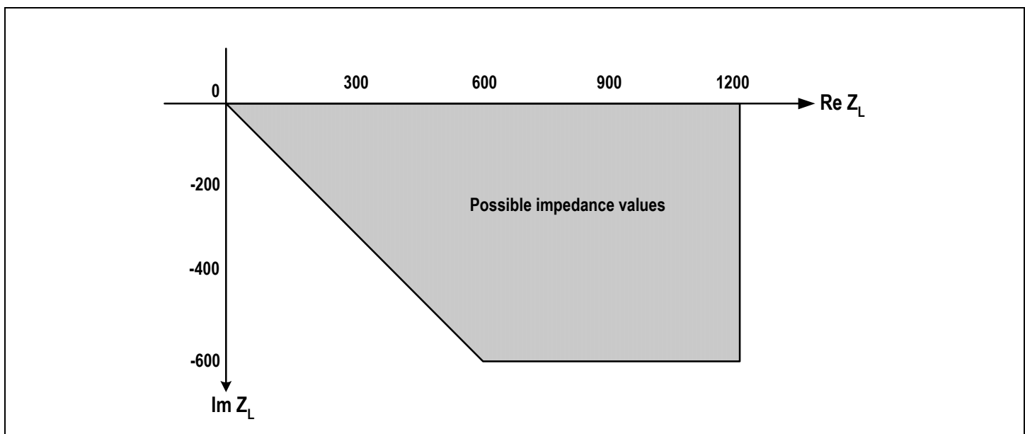
Figure - 9 Nyquist Diagram
