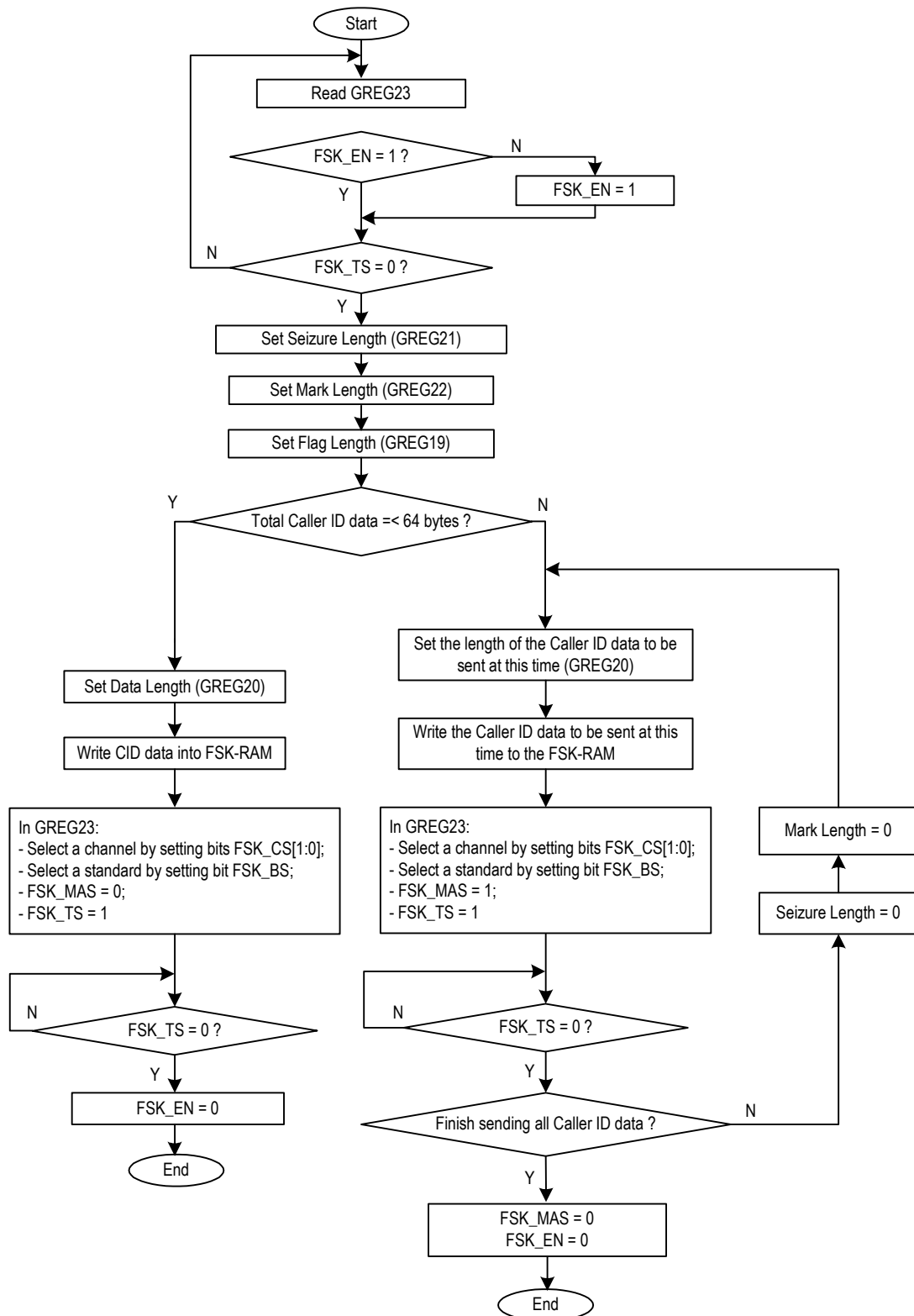
Figure - 15 Recommended Programming Flow Chart for FSK Generation
