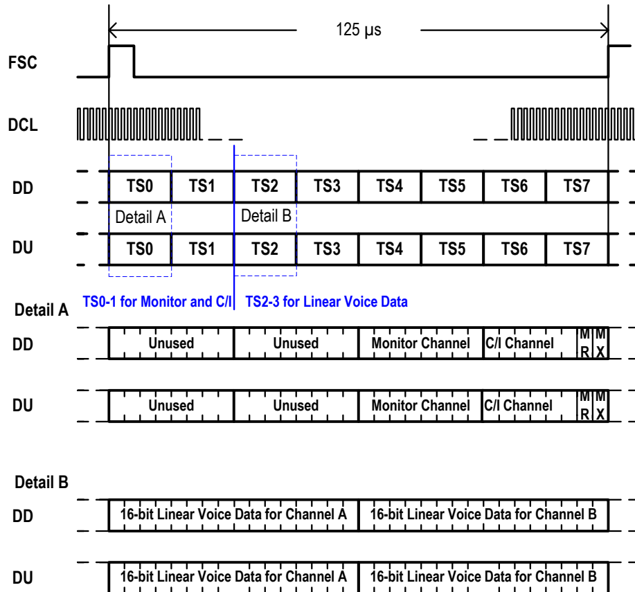
Figure - 31 Linear GCI Frame Structure
