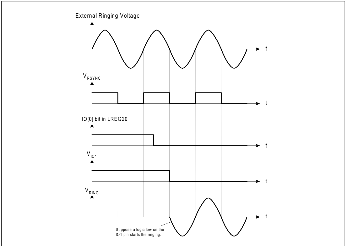
Figure - 11 External Ringing Synchronization
