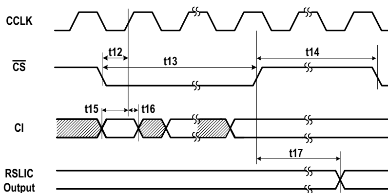
Figure - 43 MPI Input Timing
