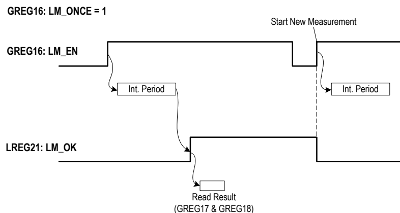
Figure - 22 Single Measurement Sequence (AC & DC Level Meter)
