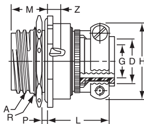
TERMINATION ASSEMBLIES "A" (SR), "E" (SR) Strain Relief
