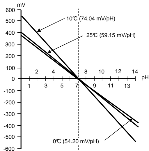
Figure 55. Temperature Dependence of a pH Electrode
