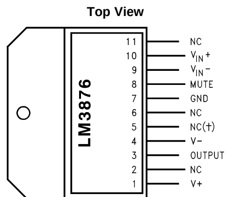
Figure 2. TO-220 and PFM Plastic Packages See Package Numbers NDJ0011B and NDA0011B (1)
