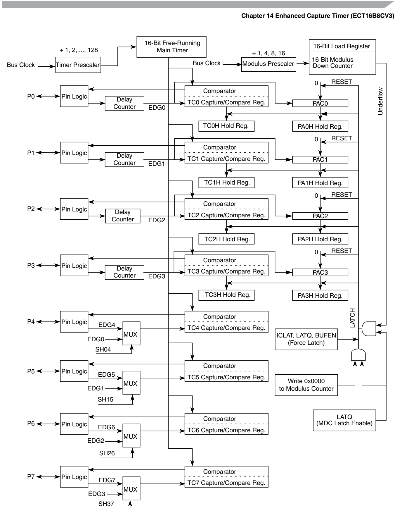
Figure 14-67. Detailed Timer Block Diagram in Latch Mode when PRNT = 0
