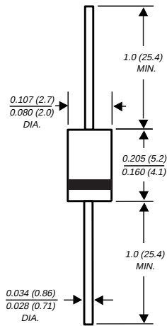
DO-204AL
