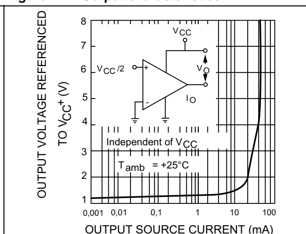
Figure 7. Output characteristics
