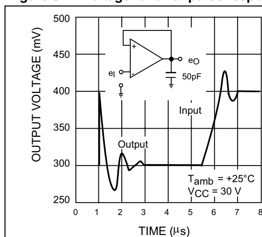
Figure 6. Voltage follower pulse response
