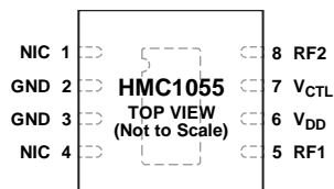
Figure 2. Pin Configuration
