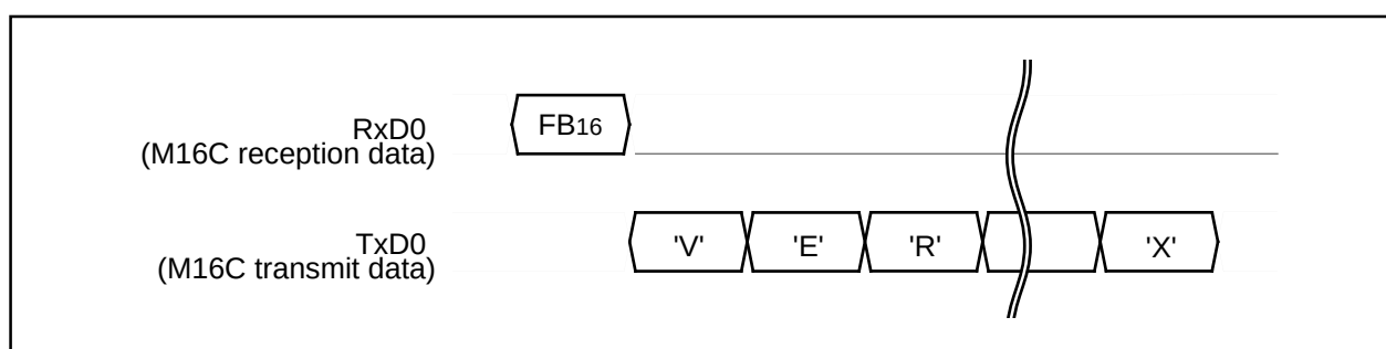
Figure 1.127. Timing for version information output
