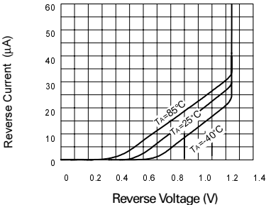
Reverse Characteristics
