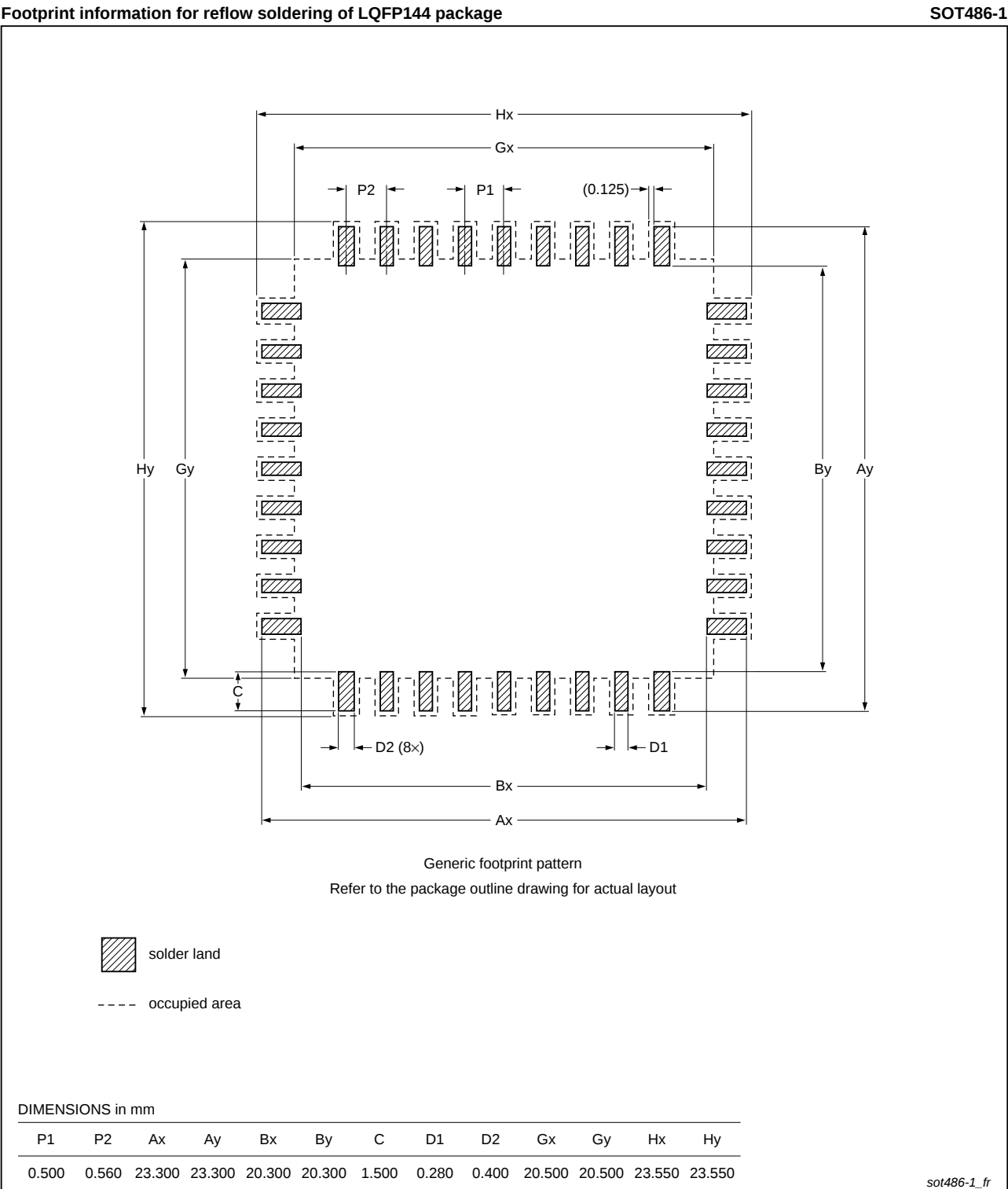
Fig 47. Reflow soldering of the LQFP144 package
