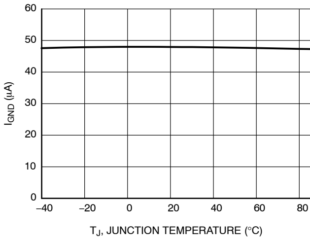
Figure 17. Supply Current vs. Temperature, 1.8 V Version
