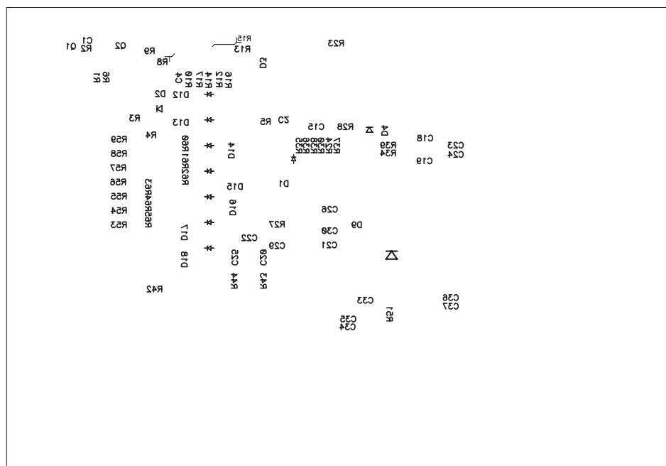
Figure 16. Bottom Silkscreen
