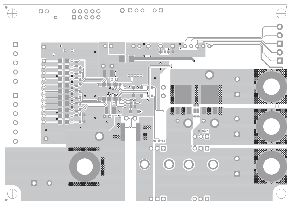
Figure 12. Top Layer
