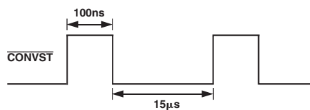
Figure 18. \overline{CONVST} When V_{IN} Channel(s) Selected
