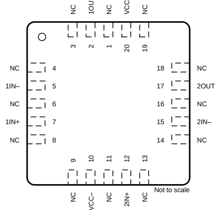
LT1013M and LT1013AM FK Package 20-Pin LCCC Top View
