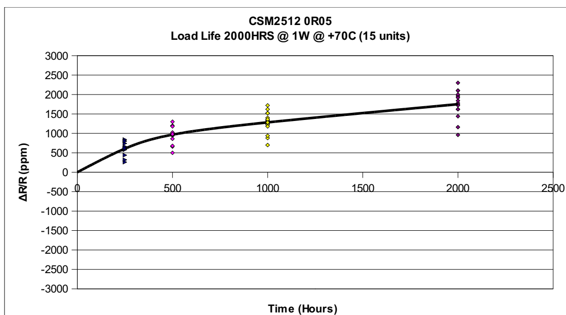
FIGURE 3 - LOAD LIFE RESULTS OF CSM2512
