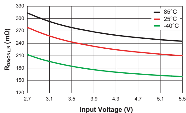
R_{\text{DS(ON)_N}} vs. Input Voltage
