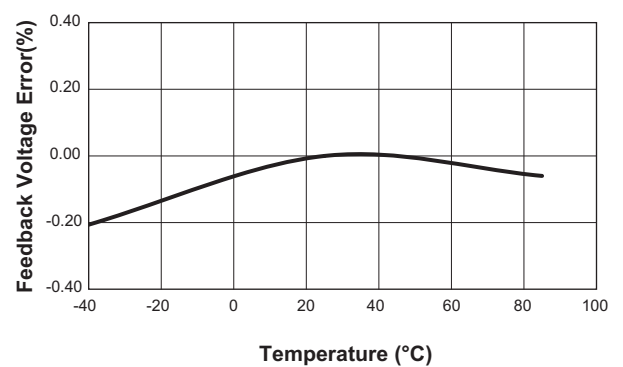
Feedback Voltage Error vs. Temperature
