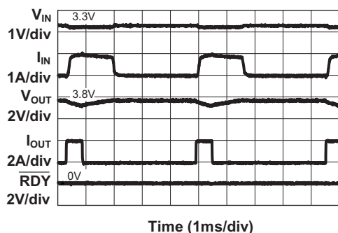
Figure 1: AAT1219 Operation Waveform When 2A 577 \mu s Load Pulse is Applied.
