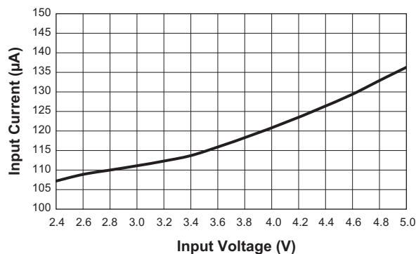
Input Current vs. Input Voltage ( V_{\text{OUT}} = 5\text{V} )
