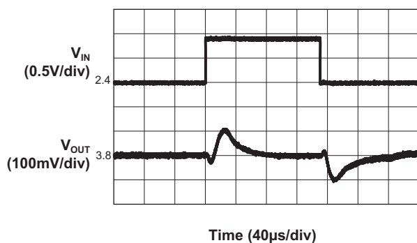
Line Transient
