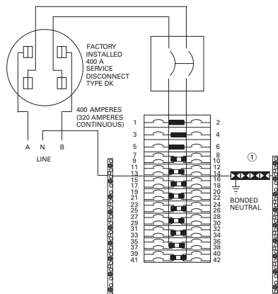
Type BR Wiring—Catalog Number HP404040SHL
