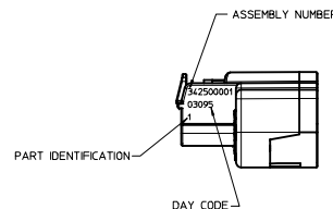
SECTION A-A TPA & CPA (OPTIONAL) SHOWN IN PRE-LOCK POSITION
