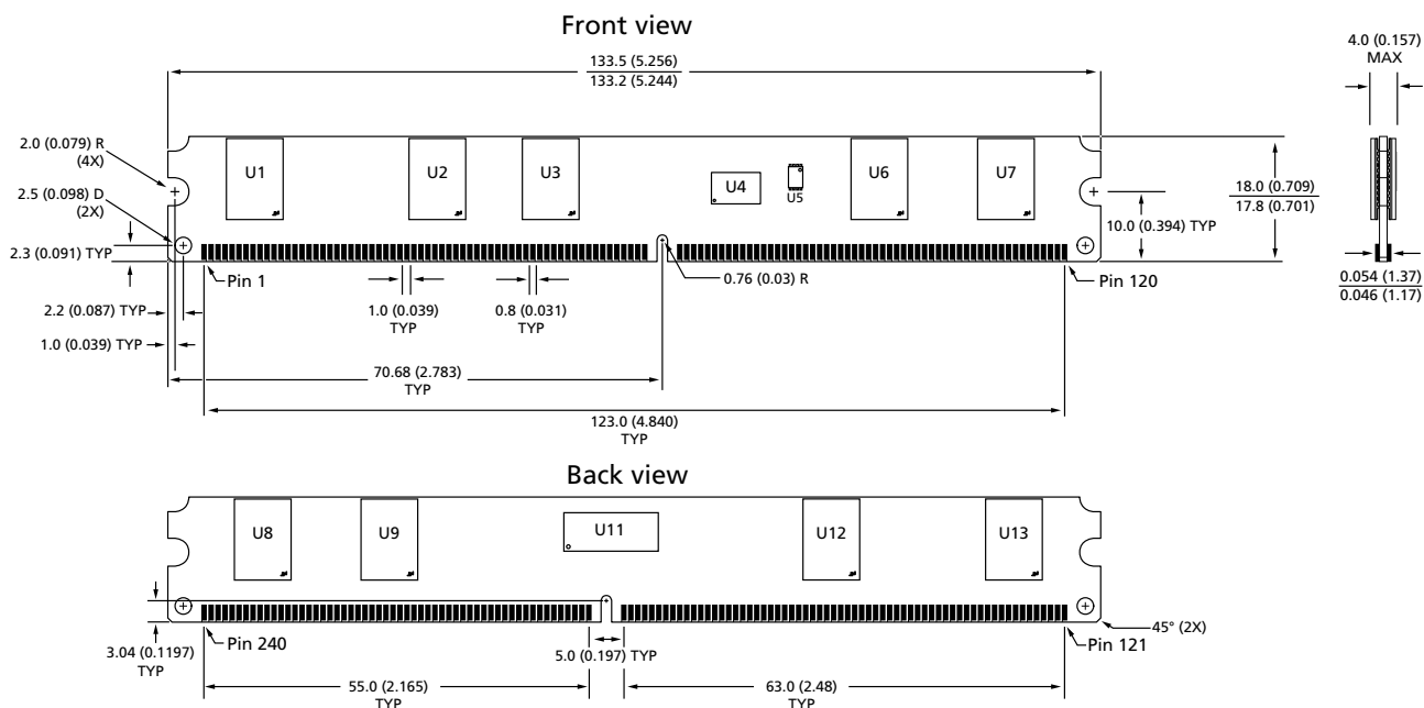
Figure 3: 240-Pin DDR2 VLP RDIMM
